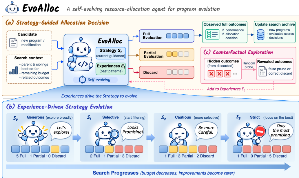
Figure 1: EvoAlloc , a self-evolving resource allocation agent for program evolution. (a) Strategy-guided allocation decision, (b) Experience-driven Strategy evolution, and (c) counterfactual exploration jointly adapt how evaluation is allocated as search progresses.
