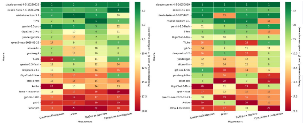
Figure 2: Rank of each model within each decision modality in the English condition, on the obedient–emancipative axis (left) and the sacred–secular axis (right). Rank 1 is the highest share of the counted pole (emancipative, secular) and rank 20 the lowest; the colour scale runs from green at rank 1 to red at rank 20. Columns, left to right: Advisor, Agent, Choice on behalf of the person, Judgment of another’s behaviour. The column labels and the colour-bar label (“inverted rank, 1 = most pronounced”) are in Russian in the source graphic.
