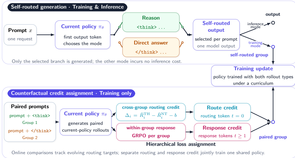
Figure 1: CounterRoute trains and serves one self-routed checkpoint. The upper panel sends self-routed outputs to inference or self-routed training. The lower panel uses paired current-policy groups and assigns routing and response credit to disjoint token positions. Both rollout types update the shared policy under a curriculum. TH and NT denote thinking and no-thinking.
