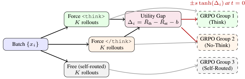
Figure 2: CounterRoute pipeline. Paired counterfactual rollouts compute per-prompt utility gaps \Delta_i , which are transformed into bounded routing advantages \pm s \tanh(\Delta_i) at position 0. Subsequent response tokens train under standard GRPO. Think, no-think, and self-routed rollout groups normalize advantages separately.
