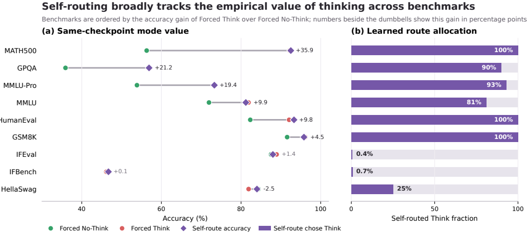
Figure 3: Same-checkpoint mode values and autonomous think rates for CounterRoute with Qwen3-8B, ordered by the forced-mode accuracy gap. Numerical results are in Appendix D.2.
