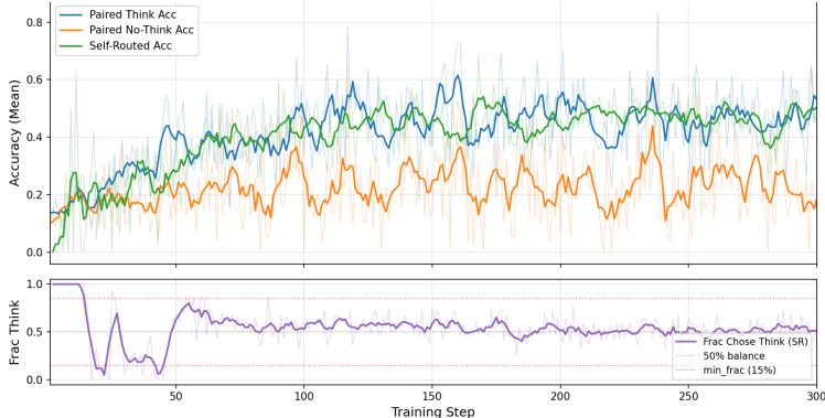
Figure 4: Qwen3-8B training dynamics on math data. The plotted accuracy is the mean correctness reward used as the task reward during training, rather than held-out evaluation accuracy. The self-routed think fraction remains non-collapsed after early exploration.
