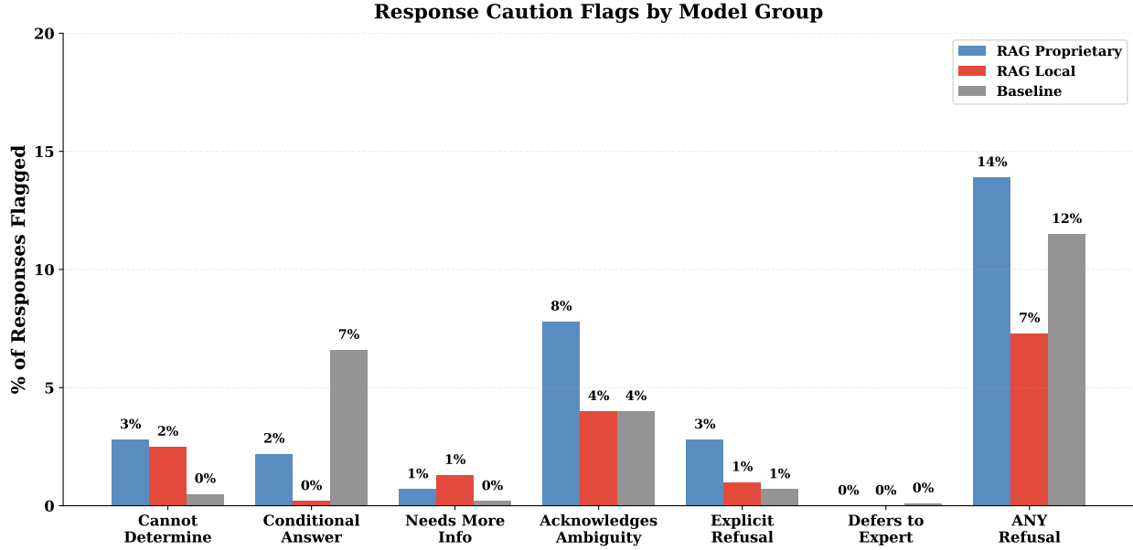
Figure 6: Ablation Study of Response Caution Flags by Model Types
