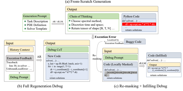
Figure 4: Illustration of from-scratch generation and debugging. (a) In from-scratch generation, models produce a CoT reasoning path and executable solver code from a generation prompt. (b) Autoregressive (AR) models repair the buggy code by full regeneration conditioned on history context and execution feedback. (c) dLLMs instead localize the buggy span from execution feedback, re-mask only the erroneous region, and repair it by infilling under full context.
