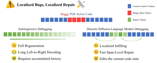
Figure 1: Comparison of debugging paradigms. AR models repair buggy solvers by sequential full-context regeneration, while DiffPDE re-masks only the erroneous region and repairs it through infilling under full surrounding context.
