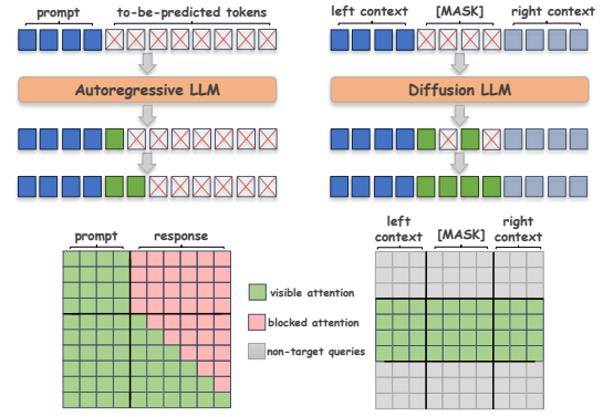
Figure 2: AR vs. diffusion debugging. AR repair typically regenerates the full solver left-to-right, whereas diffusion repair re-masks only the target span and regenerates it via iterative infilling.
