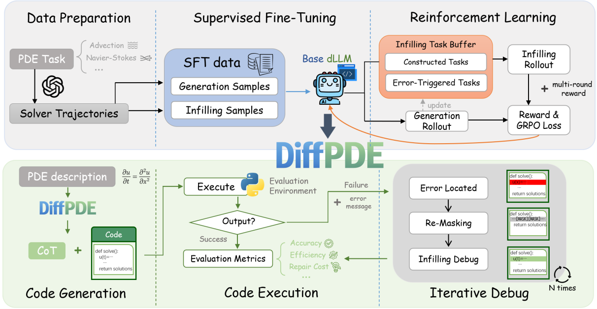
Figure 3: Overview of DiffPDE. The framework consists of a two-stage training pipeline and an inference-time iterative repair loop based on error localization, re-masking, and infilling debug.
