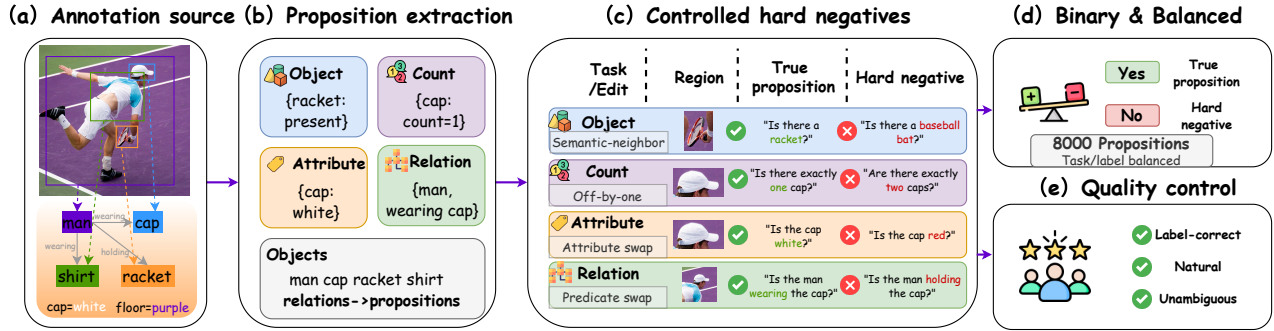
Figure 2: Construction of DYNAHALL. From COCO instances and GQA scene graphs (a), we build binary visual propositions for four tasks (b), each paired with a controlled, prior-graded hard negative (c); both polarities form a balanced set of 8,000 propositions (d) validated by expert audit (e). A single tennis scene runs through every stage.
