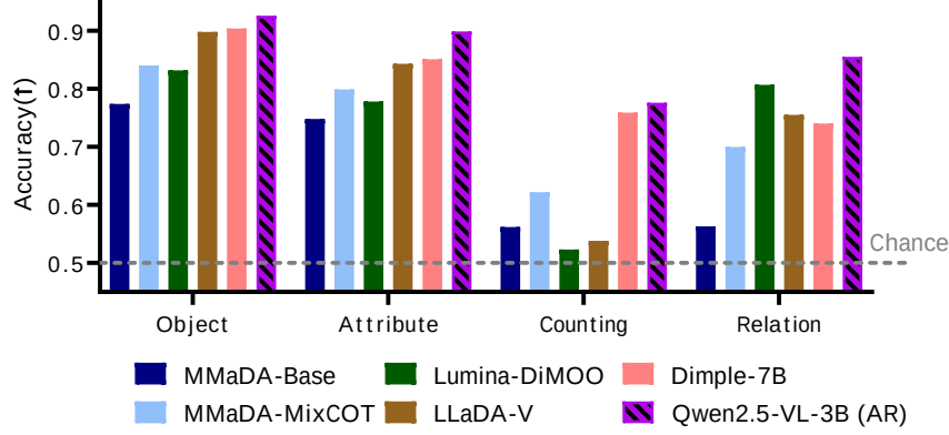
Figure 5: Per-task accuracy on DYNABALL test (7,000) for five diffusion VLMs and a strong autoregressive reference (Qwen2.5-VL-3B, hatched); the dashed line marks chance (0.5).
