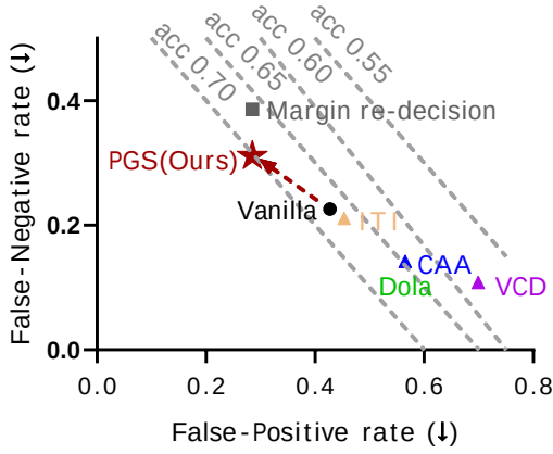
Figure 6: Operating points on DYNABALL; PGS is marked by the star. Axes show false-positive and false-negative rates; dashed lines denote iso-accuracy contours.
