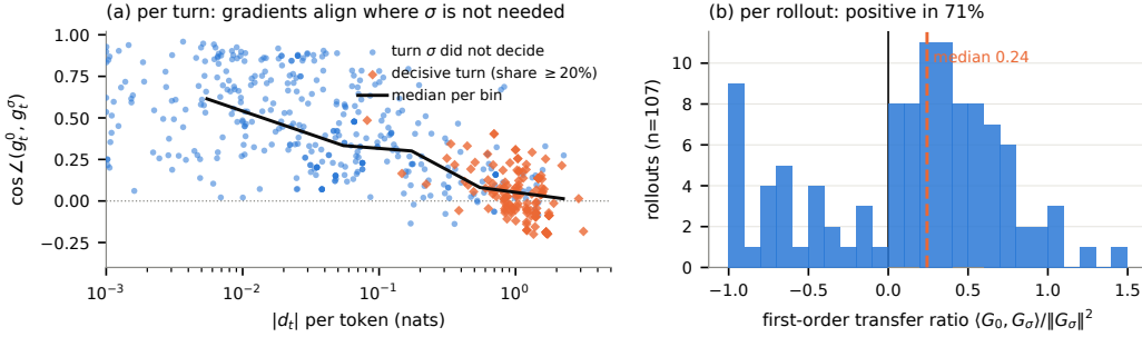
Figure 7: Measuring Proposition 1 on the base Qwen3-4B. (a) Per-turn cosine between the gradients of the two views on the same action ( \cos \angle(g_t^0, g_t^\sigma) ), against the turn’s dependence on \sigma ( |d_t| per token in Eq. (9)). Each point is one turn of a successful privileged rollout on a training task the base model does not solve. (b) The first-order transfer ratio \langle G_0, G_\sigma \rangle / \|G_\sigma\|^2 per rollout, i.e. the change in the non-privileged log-likelihood of the rollout divided by the change in the privileged one after one step. Values are clipped to [-1, 1.5] for display.
