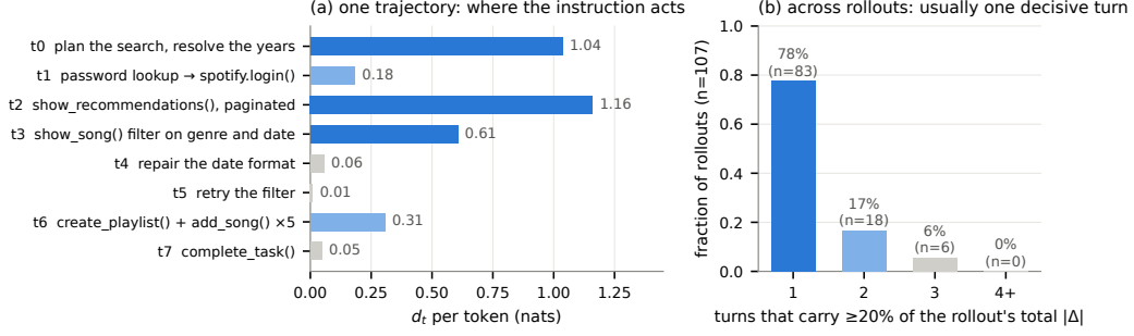
Figure 3: The instruction acts on a few turns; and the reward reinforces all of them. (a) Per-turn dependence d_t (Eq. (9)) on \sigma for one successful rollout. d_t is large where \sigma decides the action, while it's near zero where the student writes the same thing on its own. (b) Number of such decisive turns (carrying at least 20% of the rollout's total |d_t| ) across successful privileged rollouts on training tasks the base model does not solve. It's usually one and never more than three.
