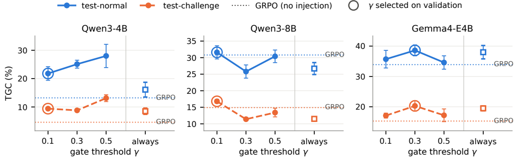
Figure 4: Effect of the gate threshold \gamma . Test TGC (mean \pm std over 5 seeds) as \gamma varies. always trains both groups for every task and doubles the rollouts per step. Dotted lines mark GRPO. Rings mark the \gamma selected on the validation set and used in Tables 1 to 3.
