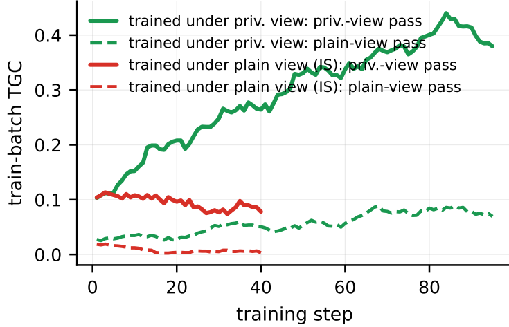
Figure 6: Identical PI-guided rollouts trained under two different views. Training the privileged view (green) can have both pass rates rise, although the non-privileged view is never trained directly. Training the non-privileged view with importance-sampling correction (red) can have both views collapse.
