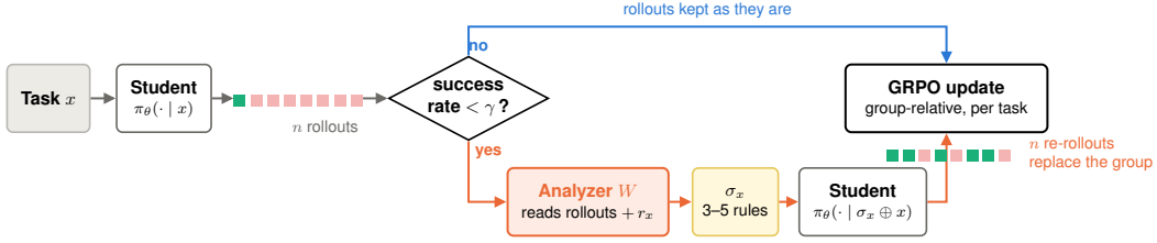
Figure 2: The framework of PSP. Each task is rolled out n times. If the group’s success rate is at least \gamma , it enters the GRPO update unchanged. Otherwise the analyzer W reads the group’s rollouts and a reference r_x , writes a short per-task instruction \sigma_x , and the task is re-rolled with \sigma_x in context.
