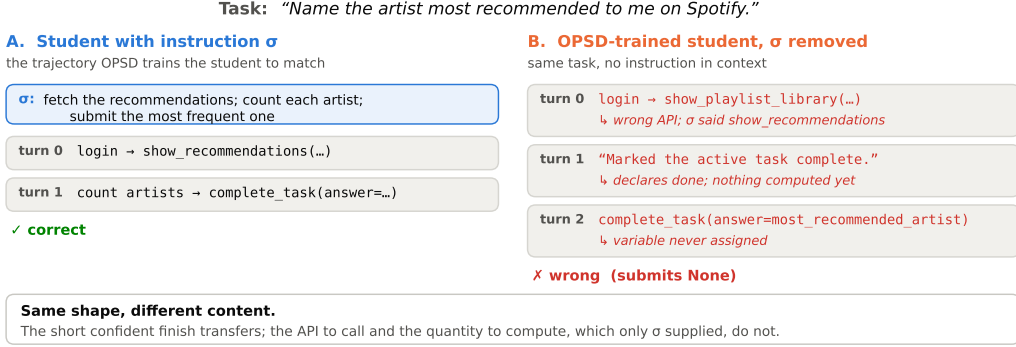
Figure 1: Matching the privileged view leaks its form but not its content. (A) with the instruction \sigma in context, the student solves the task in two turns. (B) the OPSD-trained student without \sigma reproduces the two-step shape and the closing call, but queries the wrong API, declares the task done before computing anything, and submits a variable that was never assigned.
