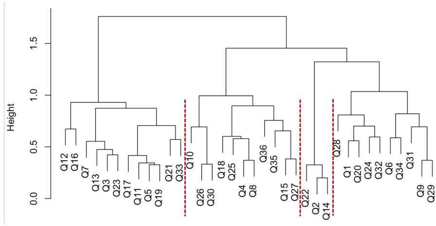
Figure II. Hierarchical cluster results for cosine similarity.
