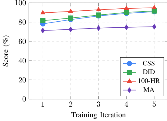
Fig. 4. Performance progression across training iterations. CSS and DID show the steepest improvements in early iterations, while gains diminish after iteration 4. The inverted hallucination rate (100-HR) demonstrates consistent safety improvements throughout training.
