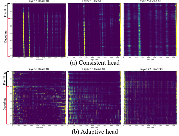
Figure 2. Visualization of attention weight heatmaps for consistent heads and adaptive heads in the LongChat-7B model using a randomly selected text segment. In these figures, the vertical axis represents the attention of the head across different queries, with the first 20 rows corresponding to the last 20 queries during the pre-filling stage, while the subsequent rows depict the attention weights across consecutive decoding steps. These two types of heads exist in layers and popular models (Appendix A).
