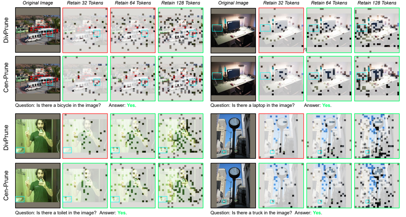
Figure A2: The case comparison of small object coverage between DivPrune and Cen-Prune from POPE.
