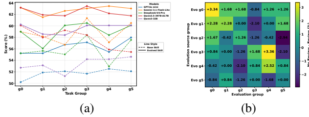
Figure 4: (a) Cross-model transfer of evolved skills on ToolQA. (b) Review ablation on ToolQA. Values denote no-review minus review accuracy.
