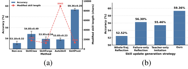
Figure 3: (a) Comparison with other skill evolution methods. (b) Comparison of skill update generation strategies.
