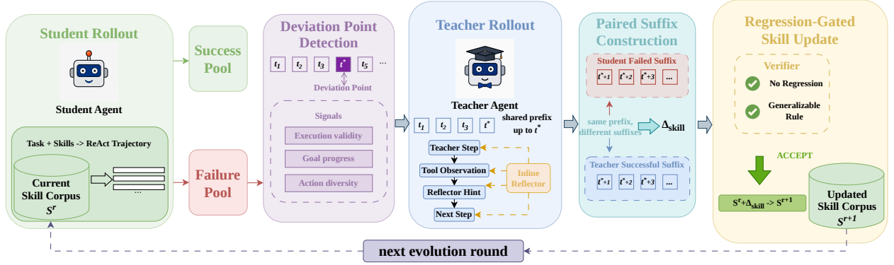
Figure 2: Overview of SkillPivot.
