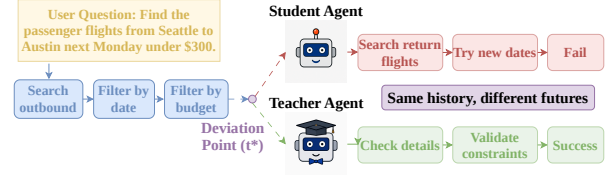
Figure 1: A failed agent trajectory can contain a useful prefix before a deviation point, and comparing the divergent suffixes from the same history reveals how the existing skill should be updated.
