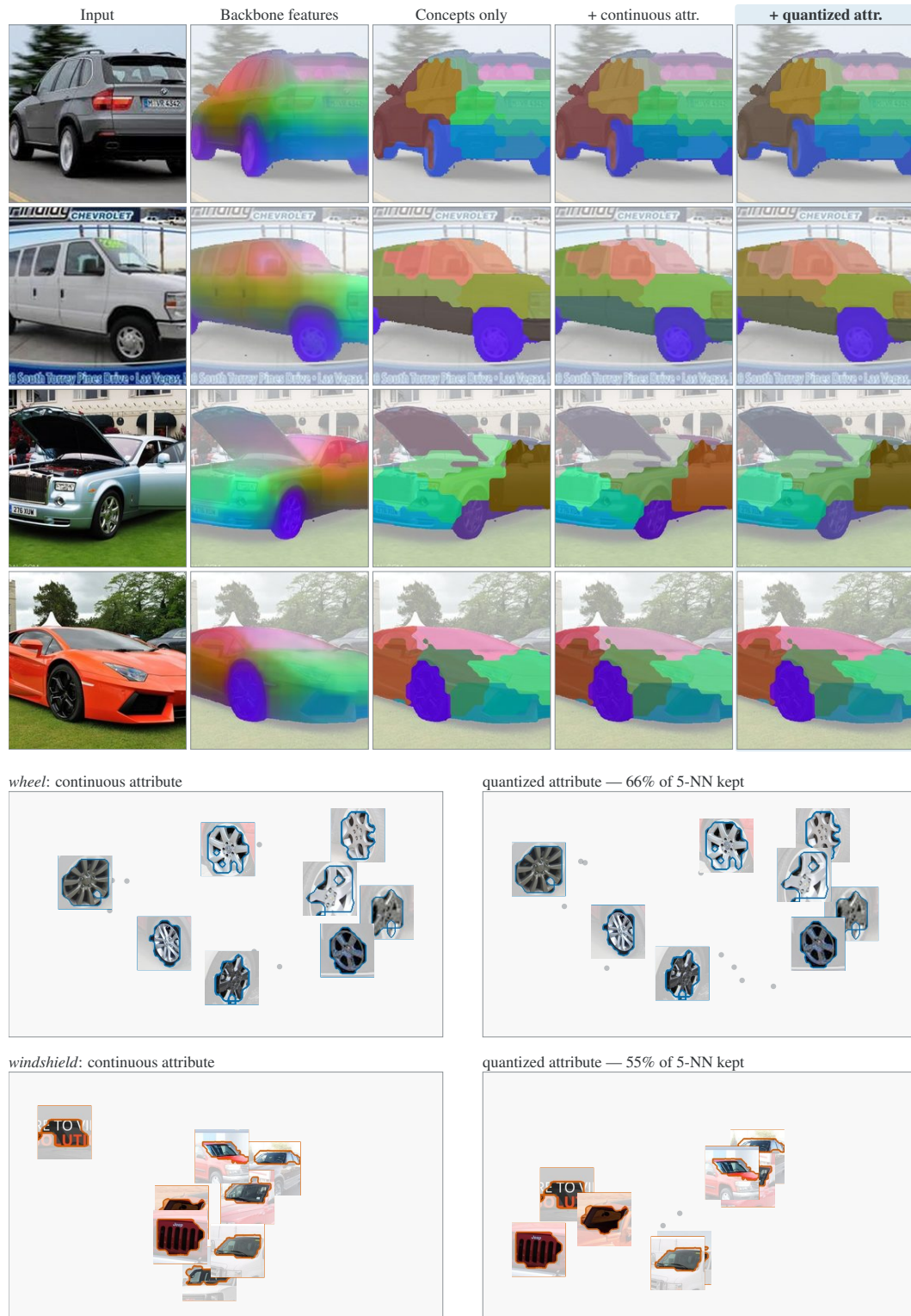
Figure 46: Stanford Cars: what quantization keeps. Top : backbone features, and each concept region as its key, key + continuous attribute and key + quantized attribute, in one PCA basis. Bottom : two concepts’ attribute spaces before and after quantization (same crops and basis; panels scaled independently).
