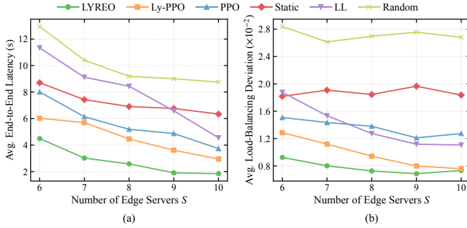
Fig. 5: Performance comparison under varying numbers of edge servers.
