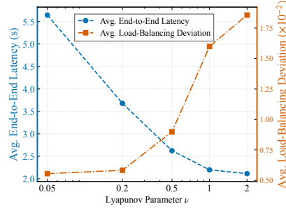
Fig. 7: Impact of Lyapunov parameter on system performance.
