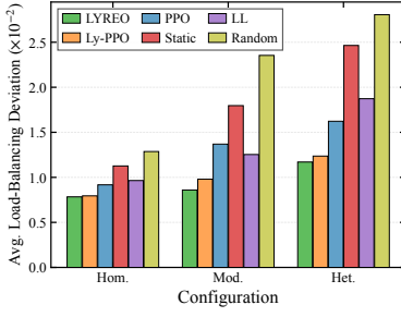
Fig. 6: Performance comparison of load-balancing deviation under varying heterogeneity levels.
