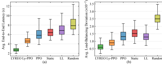
Fig. 3: Boxplot comparison of different approaches.
