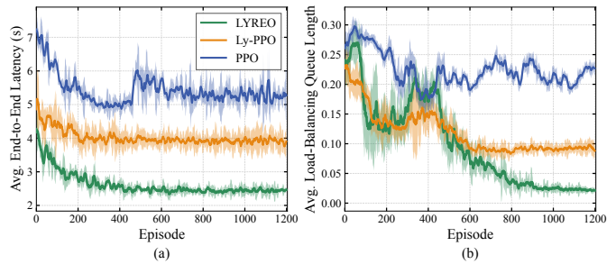
Fig. 2: Convergence performance of LYREO, Ly-PPO, and PPO approaches.
