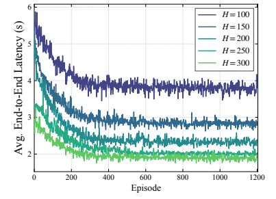
Fig. 8: Impact of truncation length on training performance.
