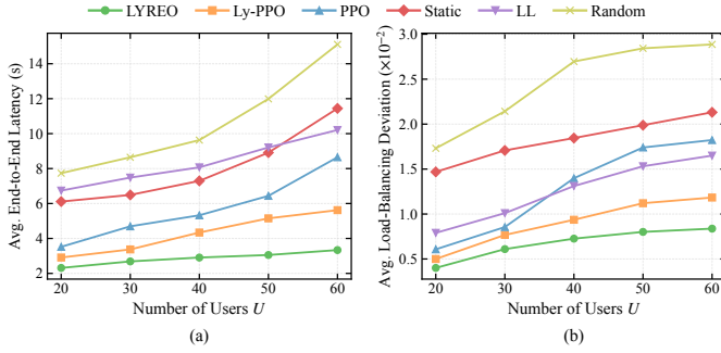
Fig. 4: Performance comparison under varying numbers of users.
