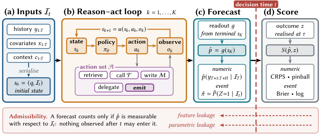
Fig. 1. Forecasting-agent pipeline corresponding to the formalism in Sections 2.3–2.4. Starting from the information set \mathcal{I}_t , the agent executes a reason-act loop and uses the readout g to produce a forecast. An appropriate forecast score evaluates the forecast when the outcome is observed at \tau . The dashed line marks decision time t , and the backward arrows show feature and parametric leakage across that boundary. Setting K = 1 and \mathcal{A} = \{\text{emit}\} yields a prompt-only zero-shot forecaster.
