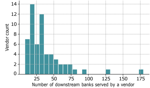
Fig. 3: Distribution of the number of downstream banks per vendor in the synthetic graph. The right tail is what makes a targeted attack on a single vendor systemically relevant.
