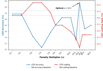
Figure 2: Hyperparameter Sensitivity: Optimizing \alpha .
