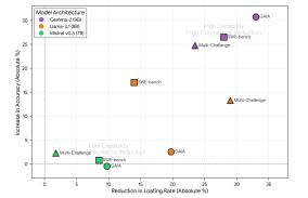
Figure 6: Compliance vs. Capability.
