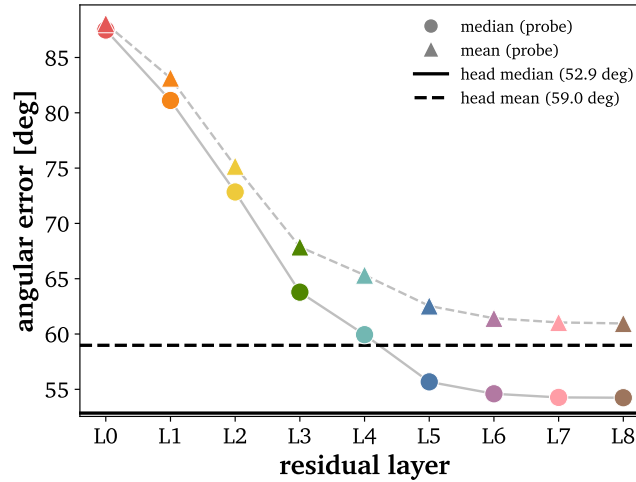
Figure 8: Held-out mean angular error of a linear CLS probe at each layer. Lower values are better; the frozen direction head is shown as a reference.
