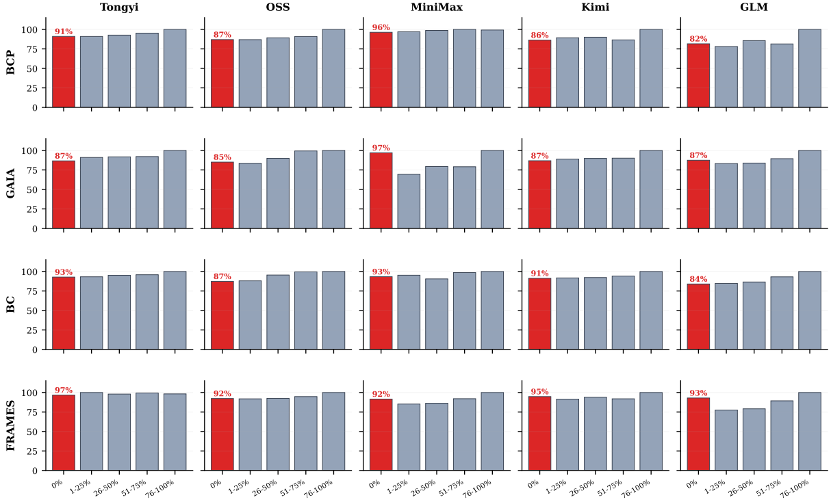
Figure 7: DeepConf overconfidence across all 20 benchmark×model cells (cf. Figure 3a). Each panel stratifies questions by oracle difficulty and reports the mean DeepConf score as a percentage of its peak. On every configuration, impossible questions (0% correct, red) receive 82–97% of the peak score. Rows: datasets; columns: models.
