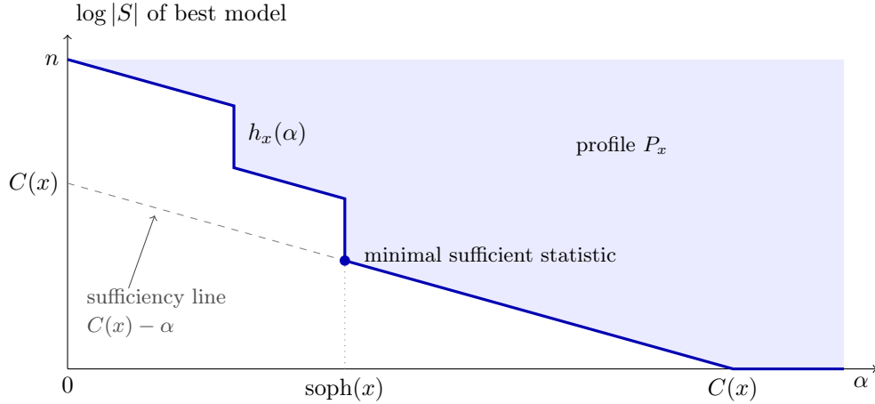
Figure 1: A typical structure function (schematic, after [11]). It lies above the sufficiency line, decreases with slope at most -1 , and touches the line first at the minimal sufficient statistic.
