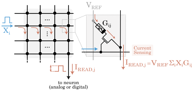
Fig. 1: An SNN with 1T1R memristive synapses employing current-mode crossbar sensing. The VMM output is represented by a column current I_{\text{READ},j} .
