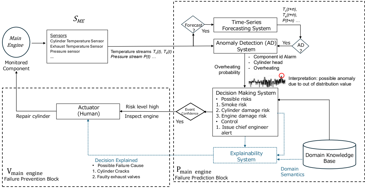
Fig. 2 Integration of the main engine component into the proposed architecture.
