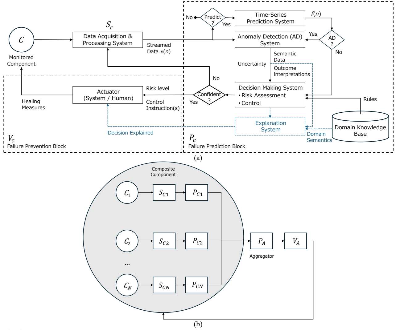
Fig. 1 Overview of the proposed conceptual architecture. (a) Monitoring of a single component of a sea vessel for failure prediction and prevention; (b) monitoring of a composite sea vessel component, considered as a system of systems.
