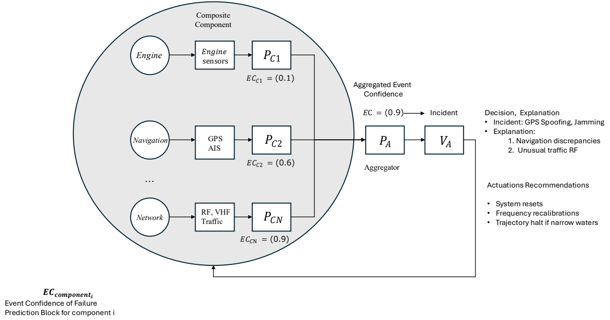
Fig. 3 The multi-component prediction-prevention loop from the proposed architecture.
