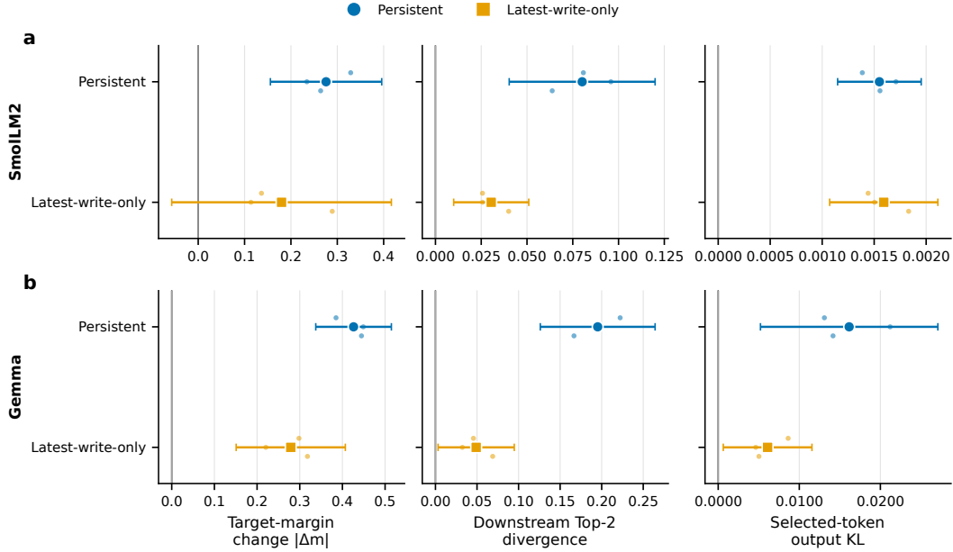
Figure 4: Downstream consequences of ledger-selected source suppression. Effects on the audited Top-2 boundary, subsequent Top-2 routing, and the selected-token output distribution for Persistent and latest-write-only. Points are three-seed means with Student- t 95% intervals ( n = 3 , df = 2 ); \cdot marks individual seeds.
