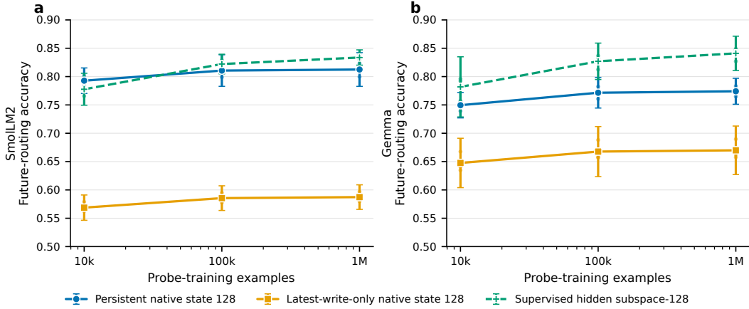
Figure 3: Compact access to future routing across training seeds. Future-router Top-1 prediction accuracy versus probe-training budget for the Persistent native state, matched latest-write-only native state, and a supervised 128-dimensional subspace of the Persistent model’s ordinary hidden stream. Points are three-seed means with Student- t 95% intervals ( n = 3 , df = 2 ); \cdot marks individual seeds.
