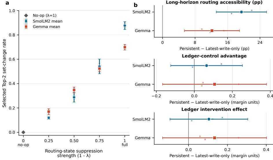
Figure 2: State use and persistence across training seeds 42/43/44. (a) Persistent-only local state-suppression dose response from Section 5.2. (b) Persistent-minus-latest-write-only contrasts for the three frozen persistence endpoints: long-horizon routing accessibility, ledger-control advantage, and ledger intervention effect. Points are three-seed means with Student- t 95% intervals ( n = 3 , df = 2 ); · marks individual seeds.
