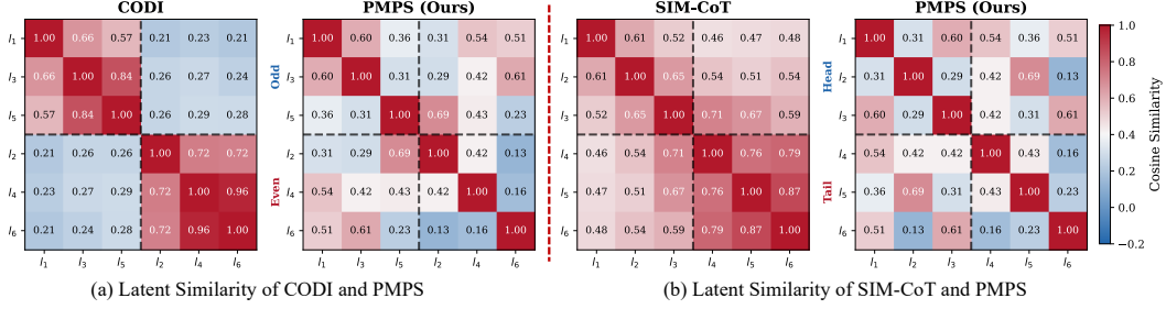
Figure 3: Average pairwise latent cosine similarity heatmaps. The latent embeddings of CODI and SIM-CoT exhibit pronounced odd-even and tail collapse, respectively, whereas PMPS shows neither pattern of collapse.
