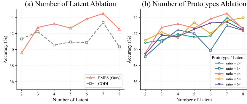
Figure 5: Ablation study on number of latent tokens and prototypes. Results are obtained with GPT-2 on GSM8K-Aug and compared against the CODI baseline.
