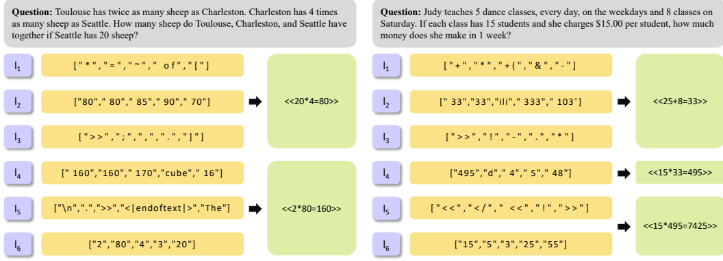
Figure 4: Interpretability cases of PMPS. We decode the latent embeddings and visualize the top-5 tokens with the highest probabilities, aligning them with the corresponding chain-of-thought (CoT) steps.
