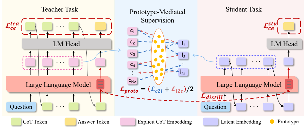
Figure 2: Overview of PMPS framework. During training, PMPS adopts the conventional parallel teacher-student architecture and leverages the explicit CoT embeddings from the teacher task to supervise the latent embeddings from the student task via a bidirectional cross-prediction loss in the prototype space. At inference, only the student task is executed, performing latent reasoning without any additional overhead.
