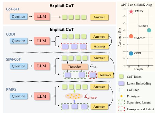
Figure 1: Comparison of different CoT methods. Our proposed PMPS provides process supervision over all latent embeddings.
