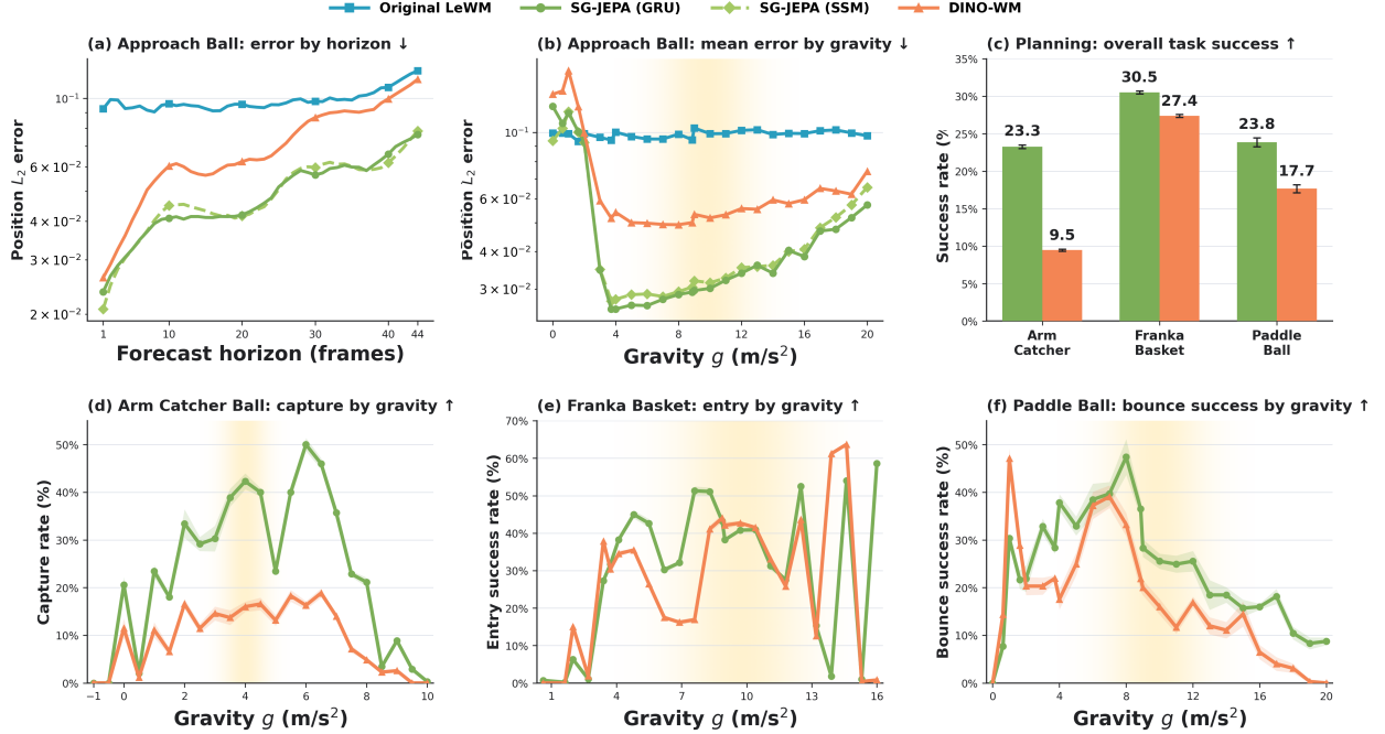
Figure 4: 3D prediction and control tasks across held-out gravity values. Open loop (a)–(b): Approach Ball position L_2 error on held-out episodes with a trained probe. Closed loop (c)–(f): Evaluation results for Diffusion Policies trained on frozen world-model features, aggregated by task and resolved by gravity (higher is better). Results are averaged over five seeds. Arm Catcher Ball and Franka Paddle-to-Basket use A = 16 , E = 8 ; Arm Paddle Ball uses A = 16 , E = 4 . Yellow shading marks the training-gravity distribution, \mathcal{N}(4, 0.5^2) for Arm Catcher Ball and \mathcal{N}(9.8, 2.0^2) for the other two.
