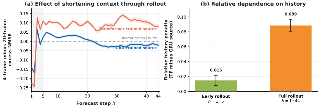
Figure 16: History dependence of the frozen representations. (a) Change in excess physical-state NMSE at each forecast step when context is shortened from H20 to H4, averaged over newly trained GRU and Transformer predictors. Positive values mean that shorter context increases error. The gray region marks the first five forecasts; bands show 95% confidence intervals over paired episode differences. (b) Transformer-source minus GRU-source history penalty over the first five forecasts and the full 44-step rollout. Positive values mean that the Transformer-trained representation depends more on long context.
