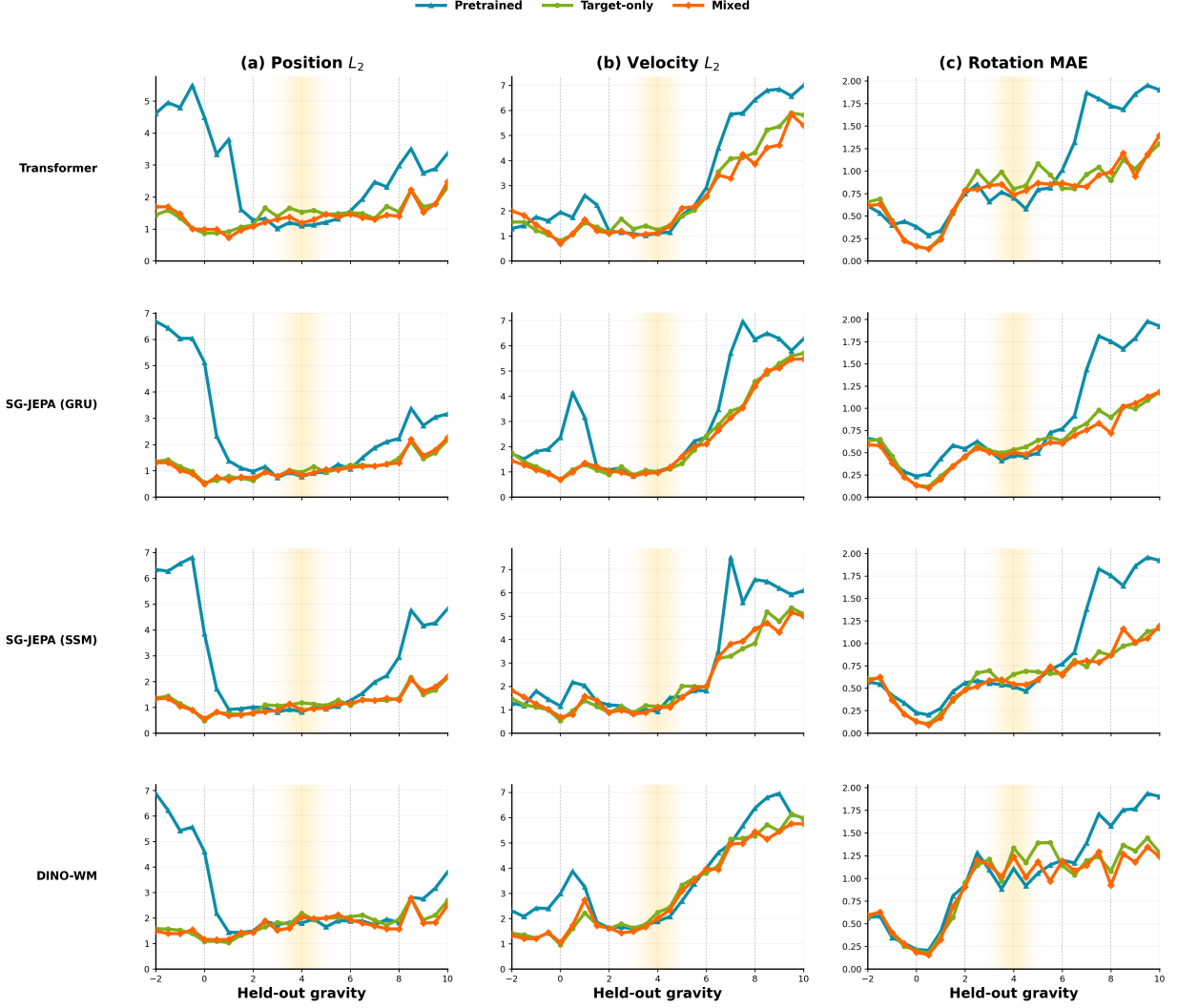
Figure 24: Right-triangle horizon-44 errors. Rows correspond to the four predictors and columns to position, velocity, and cumulative rotation. Curves show the pretrained baseline, target-only post-training, and mixed post-training over all 25 evaluation gravity values.
