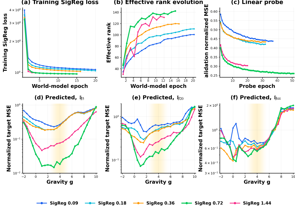
Figure 10: SIGReg coefficient sweep. (a) Raw training SIGReg loss; (b) Effective rank on the same 2,000 episodes at every checkpoint; (c) Linear-probe validation NMSE; and (d–f) MLP-probe NMSE after 5, 20, and 44 autoregressive steps across g \in [-2, 10] . Panels (c–f) use the same epoch checkpoints. The yellow shade in the background indicates training distribution. Lower is better except in (b).
