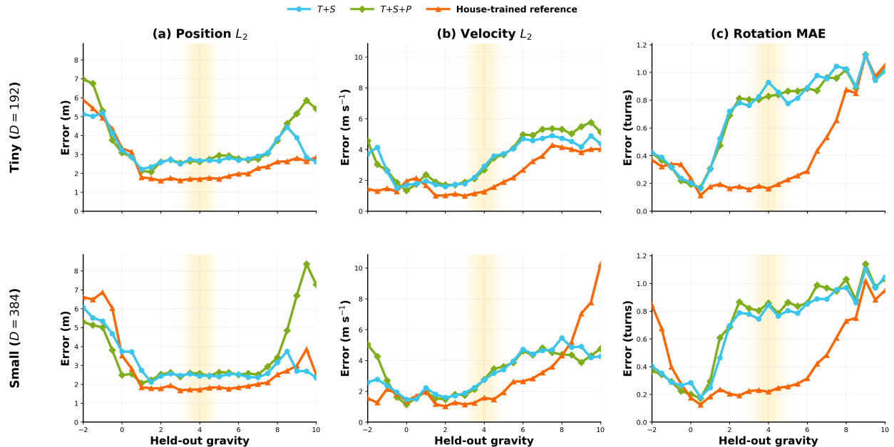
Figure 19: Per-gravity house rollout error at h_{44} . Rows show the Tiny ( D = 192 ) and Small ( D = 384 ) encoders; columns show position, velocity, and cumulative-rotation error.
