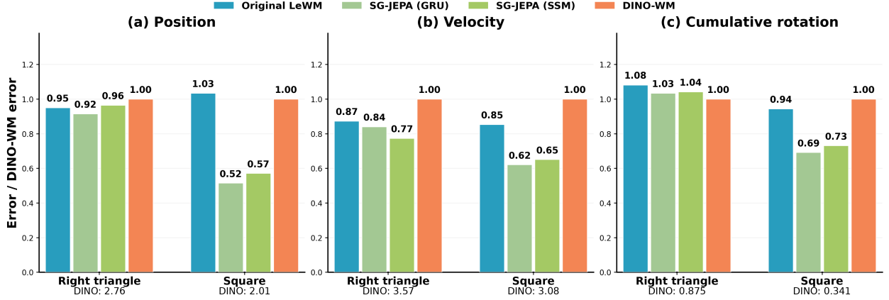
Figure 3: Long-horizon prediction at 44 rollout steps for 2D datasets, evaluated with MLP probes. Bars show position and velocity L_2 error and cumulative-rotation mean-absolute error (MAE), normalized by the DINO-WM error for each shape and metric. The absolute DINO-WM errors are shown below each group. Results are averaged over held-out episodes for each shape across 25 gravity values from -2 to 10 , with training gravity sampled from \mathcal{N}(4, 0.5^2) . Lower is better.
