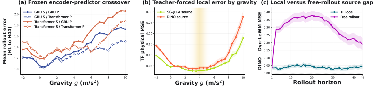
Figure 5: (a) Frozen-source predictor crossover on held-out 2D square episodes. Color denotes source; line style denotes fresh predictor. (b) Teacher-forced physical MSE from true H = 20 context, with three predictor seeds and pointwise 95% bootstrap intervals. (c) DINO-minus-Dyn teacher-forced and free-rollout gaps over 2,800 paired OOD episodes, with 95% simultaneous intervals. Positive values favor SG-JEPA.
