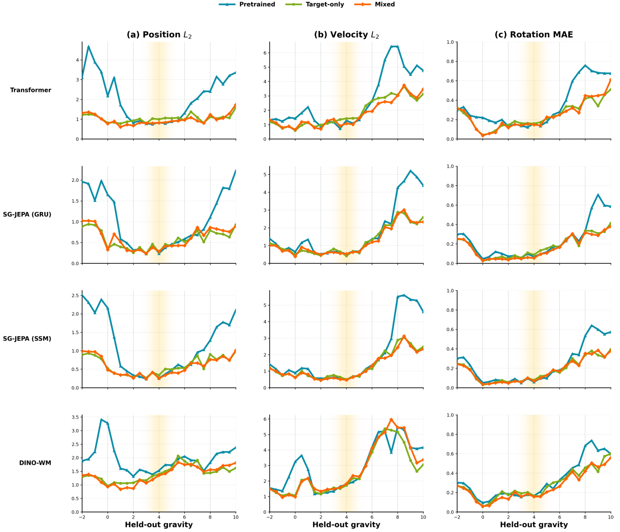
Figure 25: Square horizon-44 errors at epoch 20, using the same layout and conventions as Fig. 24.
