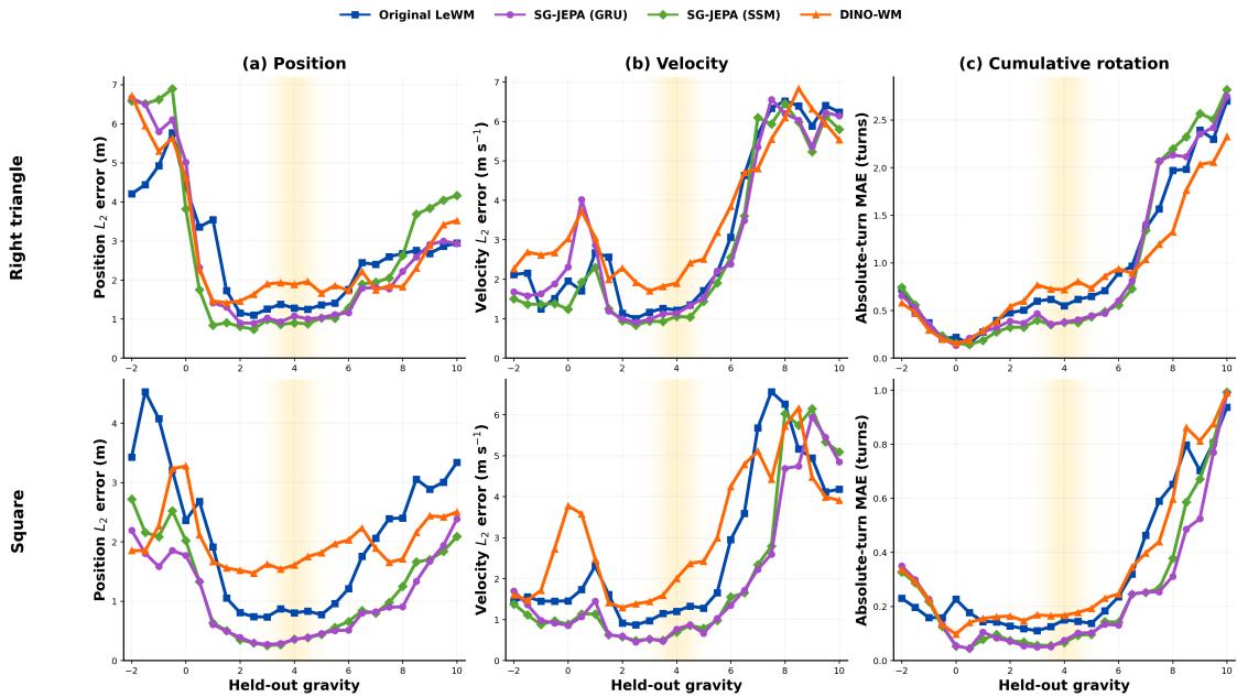
Figure 18: Per-gravity evaluation at h_{44} . Rows show right-triangle and square episodes; columns report planar position L_2 error, planar velocity L_2 error and cumulative-rotation MAE. The fading yellow background follows the relative training-gravity density g \sim N(4, 0.5^2) .
