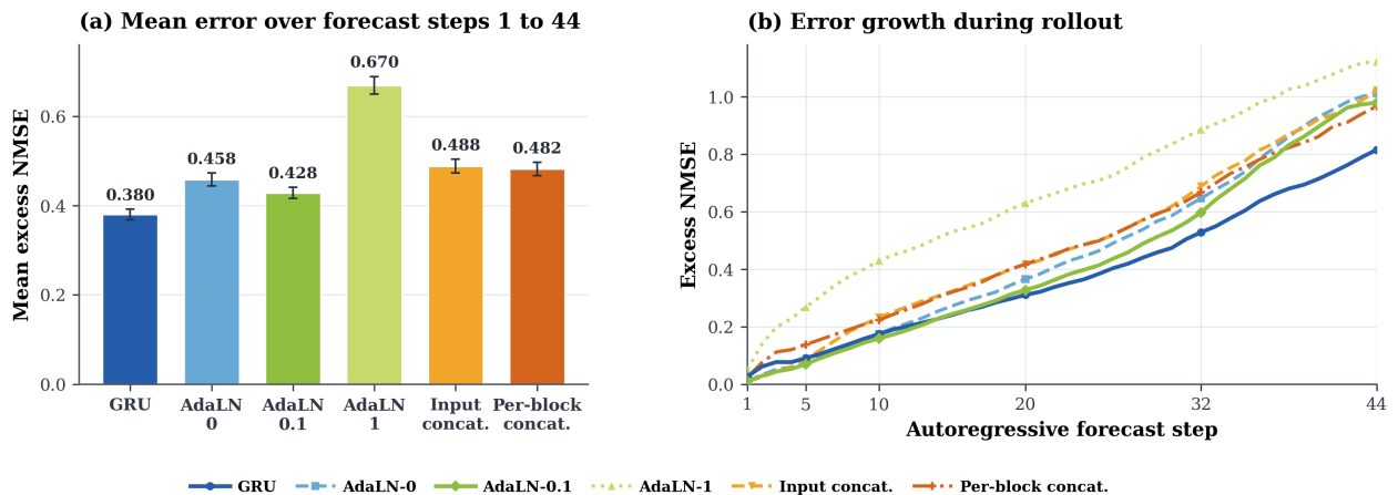
Figure 15: Performance comparison on held-out test set. (a) Mean excess normalized target MSE over forecast steps 1–44; error bars are 95% episode-bootstrap intervals. (b) Excess error by autoregressive forecast step. All models use the same episode IDs and gravity assignments. Lower is better.
