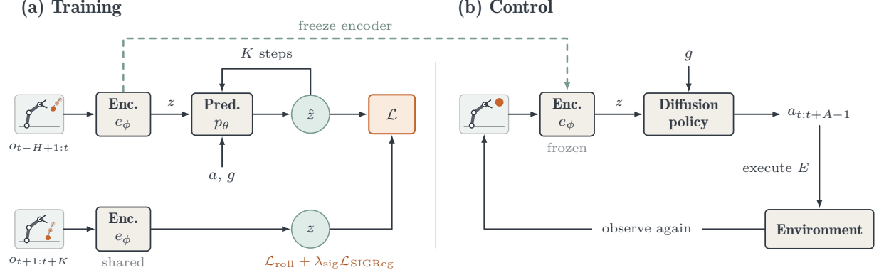
Figure 1: SG-JEPA training and control. (a) The encoder and gravity-conditioned predictor are jointly trained with a discounted K -step autoregressive rollout loss and SIGReg. Targets use the same trainable encoder. (b) A gravity-conditioned diffusion policy is trained on demonstrations from successful episodes with the encoder frozen. At inference, it generates a_{t:t+A-1} , executes the first E actions, and replans from new observations.
