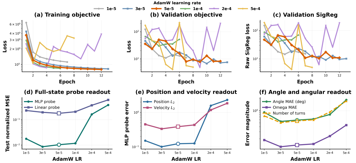
Figure 8: AdamW learning-rate sweep on 2D square dataset
