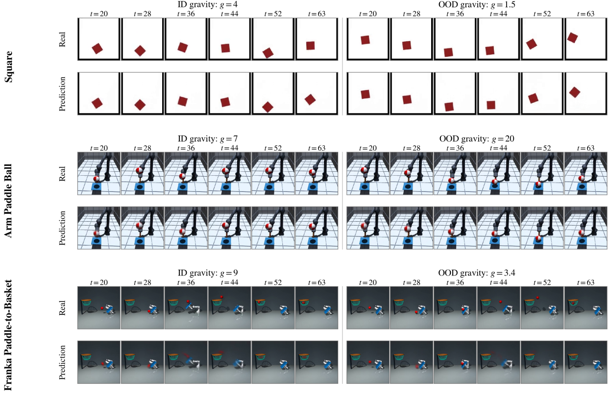
Figure 7: Decoded open-loop rollouts under in-distribution (ID) and out-of-distribution (OOD) gravity. For each dataset, the upper row shows ground-truth and the lower row decodes the autoregressively predicted latents. The model receives 20 context frames and then rolls out through t = 63 .
