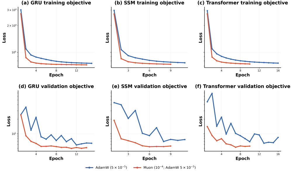
Figure 9: AdamW versus hybrid Muon/AdamW Panels (a-c) show training objectives and panels (d-f) show validation objectives for the GRU, SSM, and Transformer predictors. Lower is better.
