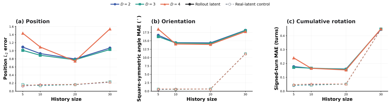
Figure 12: History-length and predictor-depth ablation on 2D square dataset at a common 32-step rollout horizon. Solid lines use predicted rollout latents; dashed lines use real encoder latents and isolate representation and probe error. Color and marker shape denote predictor depth. Lower is better.
