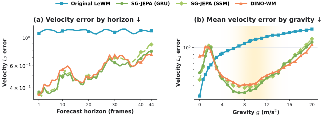
Figure 20: Approach-Ball velocity prediction. The evaluation and plotting setup matches the position results in Figure 4(a,b). (a) Mean ball-velocity L_2 error at each recursive forecast step. (b) Mean error over \mathbf{h}_1 – \mathbf{h}_{44} at each of the 25 held-out gravity values. The fading yellow background shows the training distribution g \sim \mathcal{N}(9.8, 2.0^2) .
