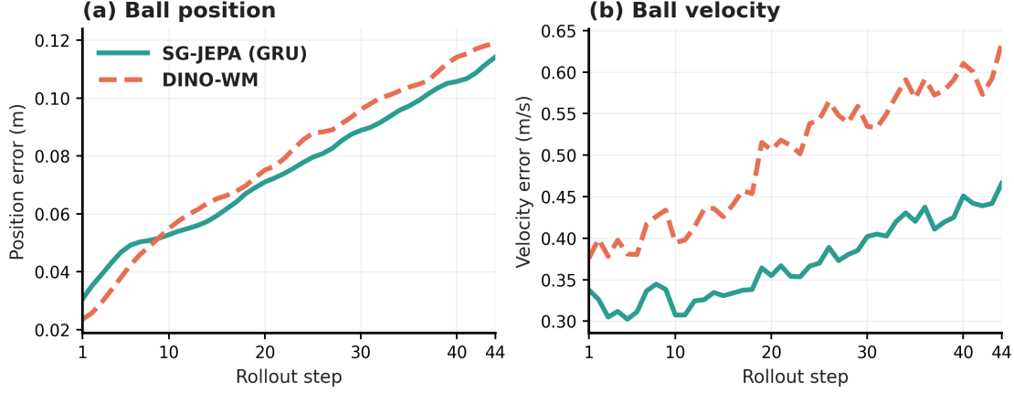
Figure 23: Open-loop Arm-Paddle-Ball prediction. Mean Euclidean error for (a) ball position and (b) ball velocity over 5,000 held-out episodes. SG-JEPA has lower position error from \mathfrak{h}_9 onward and lower velocity error at every forecast step.
