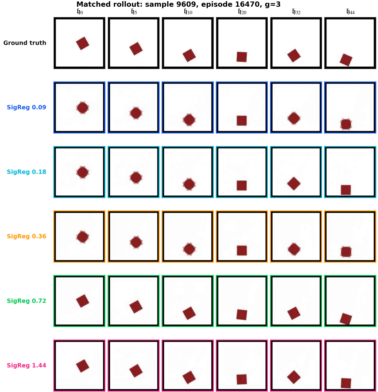
Figure 11: Qualitative comparison of the SIGReg coefficient. Matched rollout predictions for one representative square episode at g = 3 . The top row shows ground-truth frames, and the remaining rows show decoded predicted latents for each value of \lambda_{\text{SIG}} . Columns show the autoregressive rollout horizons 5, 10, 20, 32 and 44. Each prediction row is rendered using the online decoder trained jointly with that model.
