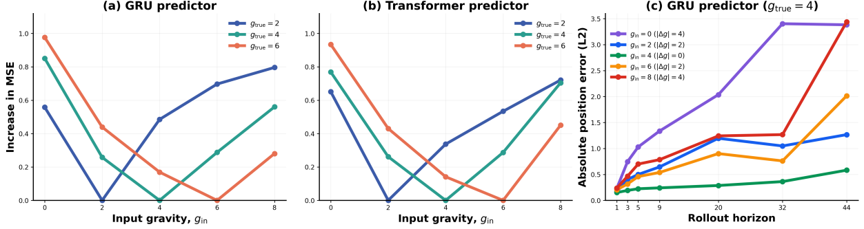
Figure 14: Counterfactual gravity conditioning Only the gravity supplied through the action channel is changed. Panels (a) and (b) report the increase in normalized full-state probe NMSE AUC for the GRU and Transformer predictors. Panel (c) reports the mean GRU position L_2 error in the x - z plane across rollout horizons for g_{true} = 4 .
