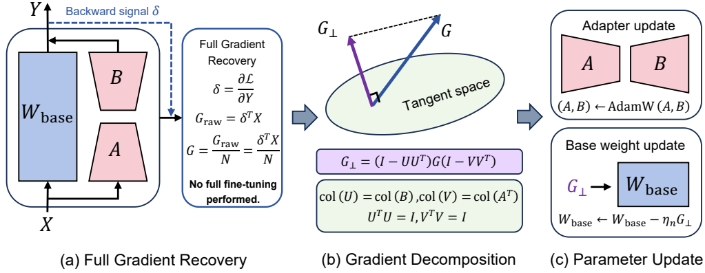
Figure 1: Overview of GDLORA. (a) GDLORA reconstructs the full weight gradient at the current model parameters from forward activations and backward signals, and obtains G as defined in Section 3.1. (b) The gradient is decomposed with respect to the current parameterization-induced LoRA tangent space, and its orthogonal component G_{\perp} is the normal gradient . (c) The adapters follow standard AdamW optimization, while G_{\perp} updates W_{\text{base}} without additional base-weight momentum or variance buffers. The two branches are complementary at first order at the current iterate.
