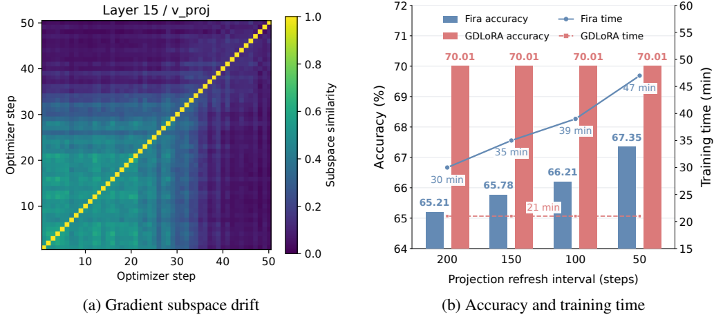
Figure 3: Gradient subspace drift and projection refresh costs. (a) Pairwise similarity between the leading rank-8 gradient subspaces of model.layers.15.self_attn.v_proj over 50 optimizer steps. (b) Accuracy and training time of native Fira with projection refresh intervals of 200, 150, 100, and 50 steps on Math10K with Llama-3-8B. GDLORA is shown as a fixed reference; its repeated values correspond to the same configuration.
