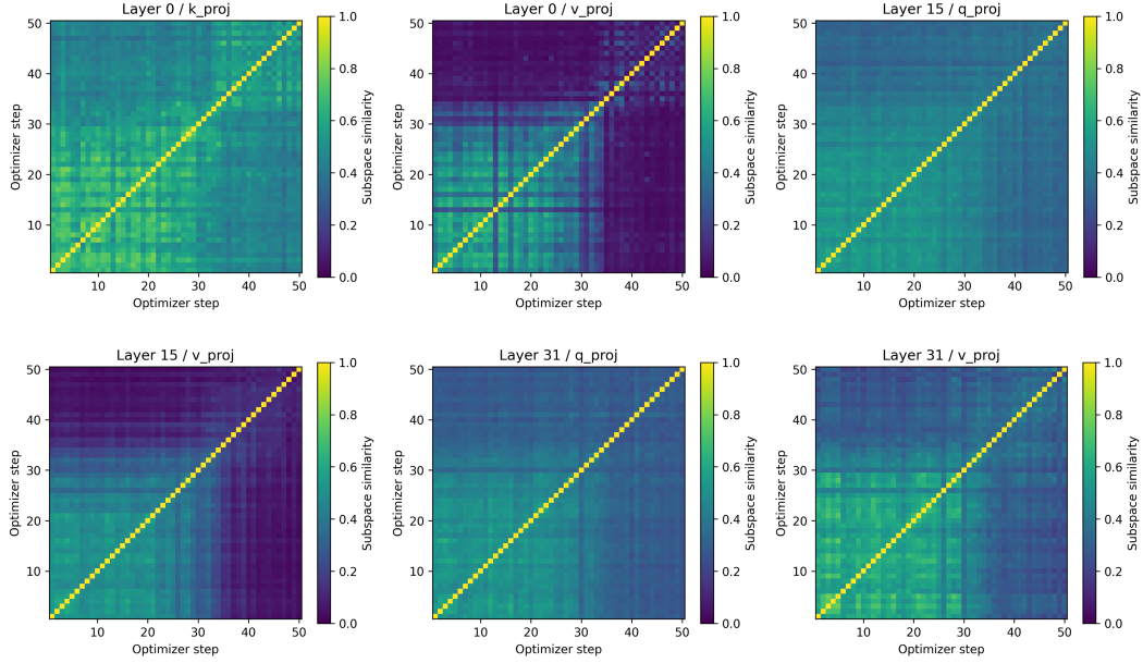
Figure 4: Gradient subspace variation across network depths and attention projections. Each heatmap shows pairwise similarity between leading rank-8 gradient subspaces over 50 optimizer steps during Llama-3-8B fine-tuning on Math10K. From left to right, the top row shows the layer-0 key, layer-0 value, and layer-15 query projections; the bottom row shows the layer-15 value, layer-31 query, and layer-31 value projections. Layer numbers follow the model’s module indices. The layer-15 value projection is also shown in Figure 3(a). All panels use the same color scale.
