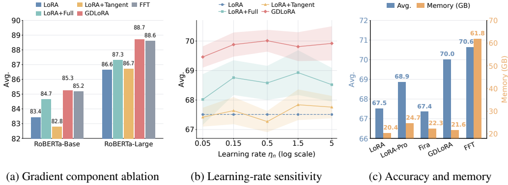
Figure 2: Ablation studies and analysis of GDLORA. (a) Comparison of gradient components on six GLUE tasks with RoBERTa-Base and RoBERTa-Large. (b) Sensitivity to the base-update learning rate when fine-tuning Llama-3-8B on Math10K. Shaded bands indicate \pm 1 standard deviation. (c) Average mathematical reasoning accuracy and memory usage with Llama-3-8B on Math10K.
