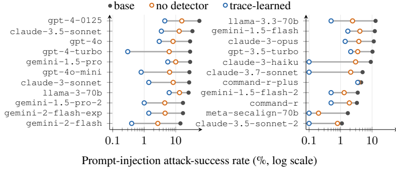
Figure 5: Indirect prompt-injection prevention across 22 LLMs on AgentDojo; left and right are the higher- and lower-ASR halves.
