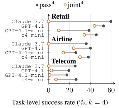
Figure 6: The \tau^2 -bench procedural reliability across three domains and four models.
