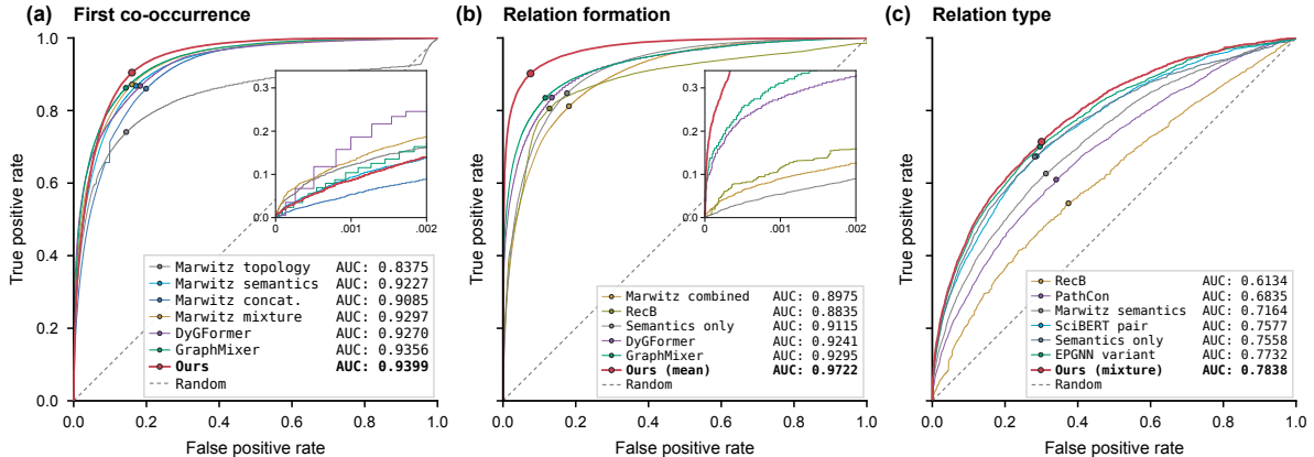
Fig. 2. ROC curves: (a,b) population weighted; (c) mean of three one-vs-rest curves. Our relation curve is the mean ROC from the three refreshed checkpoints in Tables 1 and 2; other curves show representative runs. Insets magnify low false-positive rates.
