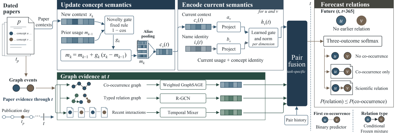
Fig. 1. Time-aligned evolving concept graphs. Dated papers provide contextual occurrences and graph events through query time t . Reconstructed semantic and structural states are fused at the concept-pair level to forecast first co-occurrence, relation formation, and conditional relation type.
