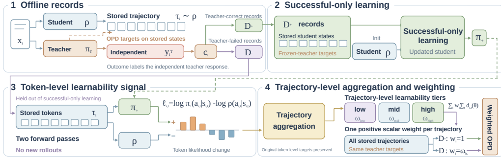
Figure 2: Learnability-Weighted Distillation (LWD) for offline OPD. (1) We collect student trajectories, frozen-teacher targets, and outcomes of independently generated teacher responses. (2) Teacher-successful records train a reference checkpoint \pi_+ from \rho . (3) Stored trajectories from teacher-failed problems are rescored under both checkpoints, and their token-level likelihood changes are summarized by the trajectory mean and variation. (4) The resulting tiers assign bounded positive trajectory weights for final offline distillation. Scoring uses two forward passes and no new rollouts. The token profile is schematic; the displayed weights are realized Code values.
