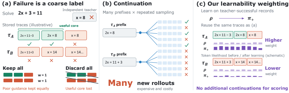
Figure 1: Motivation for learnability-weighted OPD. (a) A failed teacher response provides only a problem-level label. Student trajectories with the same label may deserve different amounts of OPD supervision. Keeping all weights them equally, while discarding all can remove useful supervision. (b) Estimating recoverability requires repeated continuation and verification from many prefixes. (c) We compare stored-token likelihoods before and after successful-only learning to assign positive trajectory weights. This requires no repeated continuation rollouts from multiple prefixes.
