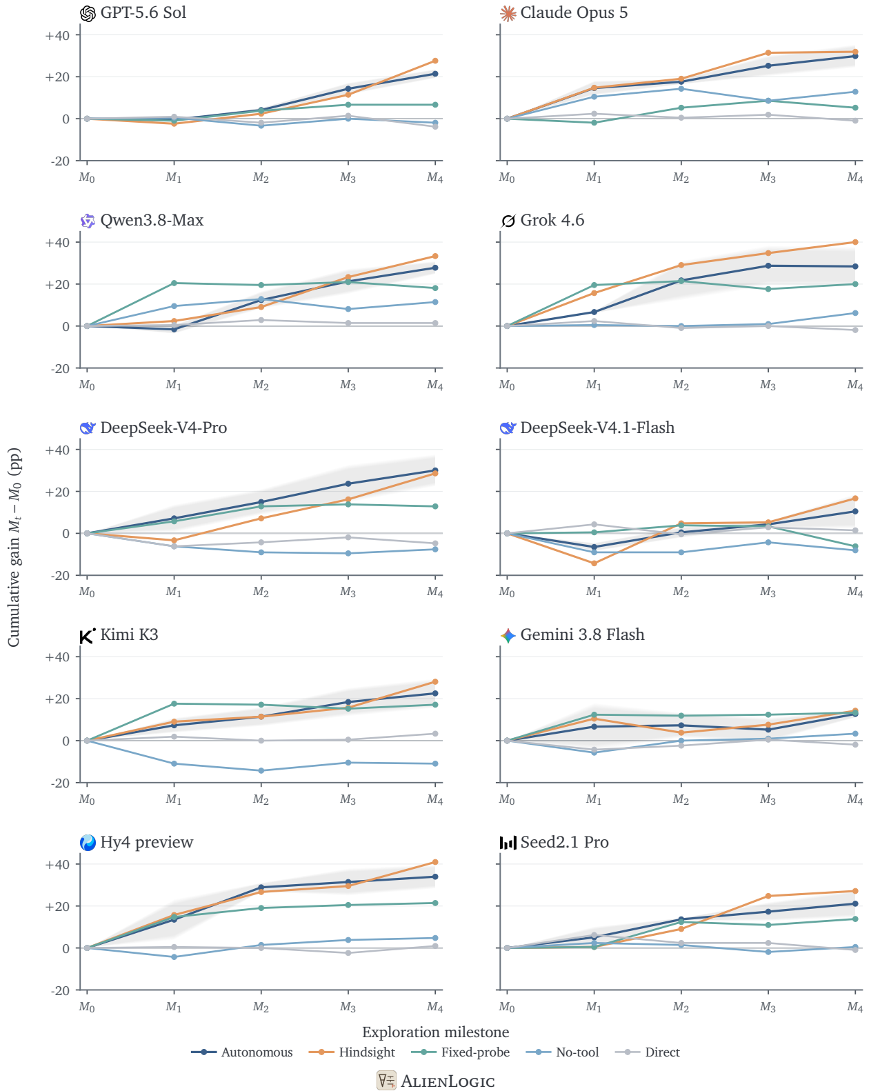
Figure 14 | Exploration trajectories for every ALIENLOGIC system. Curves show cumulative gain M_t - M_0 . The autonomous curve is the mean of three trajectories, and its shading is \pm population SD across them; each control curve is a single trajectory.
