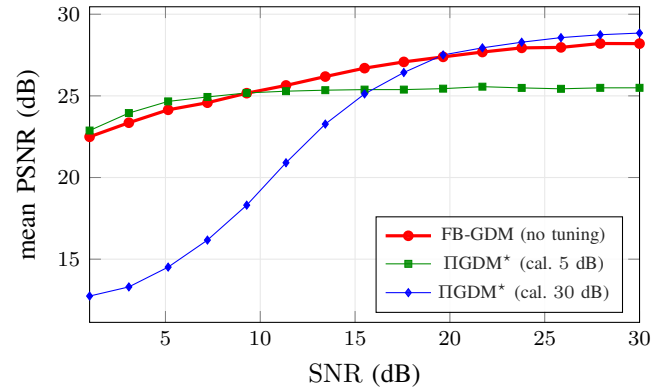
Fig. 4. Robustness to the signal-to-noise ratio on super-resolution \times 4 , SNR swept from 1 to 30 dB. FB-GDM uses no tuning; each \Pi\text{GDM}^* curve is calibrated on the ground truth at a single SNR, then frozen.
