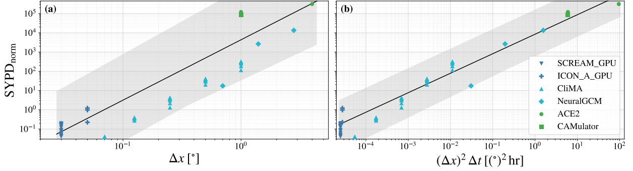
Figure 9: Reported normalized throughput across GPU-accelerated dynamical, hybrid AI-physics, and AI emulator models. Each point represents one reported model configuration. Panel (a) plots \text{SYDP}_{\text{norm}} against nominal horizontal grid spacing \Delta x , whereas panel (b) accounts for the reported prognostic update time-interval through (\Delta x)^2 \Delta t ; both panels share the same ordinate scale. Black lines are descriptive weighted-least-squares fits in log-log space, assigning equal total weight to each model. Gray envelopes are nominal 95% prediction intervals.
