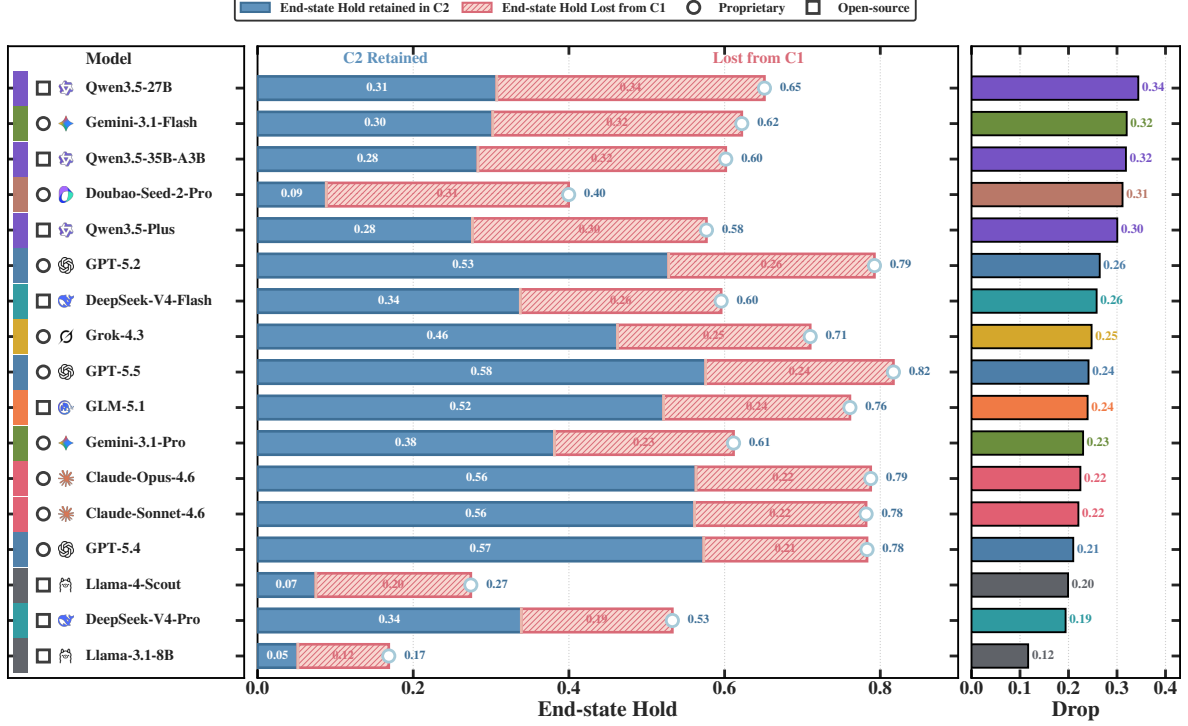
Figure 4: End-state Hold under single-turn and multi-turn narration ( C_1 and C_2 ). Solid bars show EH retained under C_2 ; hatched bars show the portion lost from C_1 . The right panel reports the drop in percentage points.
