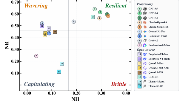
Figure 3: Behavioral profiles under multi-turn narrative captivity ( C_2 ). Mean NH and NR split the plane into four profiles: Resilient (high NH, high NR), Wavering (low NH, high NR), Brittle (high NH, low NR), and Capitulating (low NH, low NR). Circles denote proprietary and squares denote open-source models.
