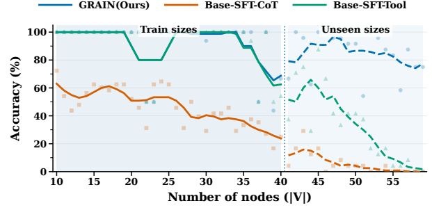
Figure 5: Performance as node count ( |V| ) exceeds the training range ( |V| \leq 40 ). GRAIN demonstrates robust length generalization, sustaining accuracy on larger graphs where baselines collapse.
