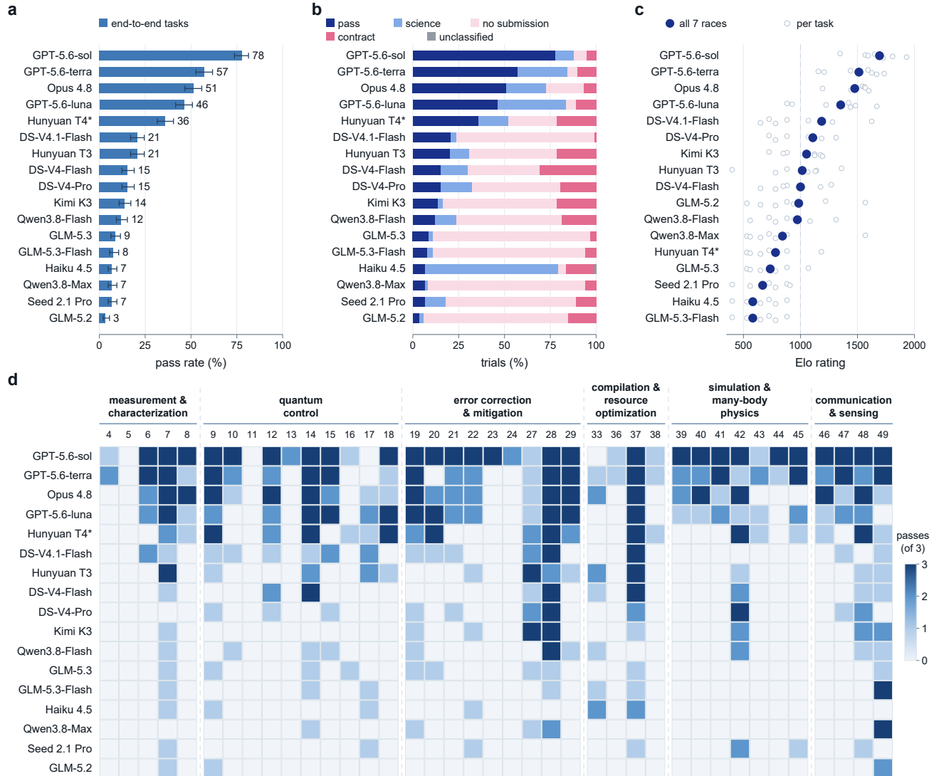
FIG. 4. Benchmark results and analysis of failure and pass patterns. a. Pass rate on the pass-fail tasks. Error bars: Wilson 68% intervals. b. Outcome composition of the trials, including passes, science failures, contract failures, and no-submission trials. c. Bradley-Terry Elo ratings over the 7 racing tasks (filled circles: games-weighted aggregate; open circles: per-task ratings). d. Per-task passes for every system, grouped by the scientific categories of Fig. 3, easiest to hardest within each group. Only pass-fail tasks are shown here.
