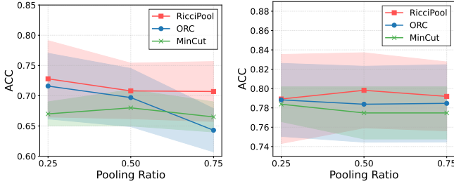
Fig. 4: Comparison under different pooling rates with the same Ollivier-Ricci flow iteration l = 5 (left: IMDB-B, right: PROTEINS).
