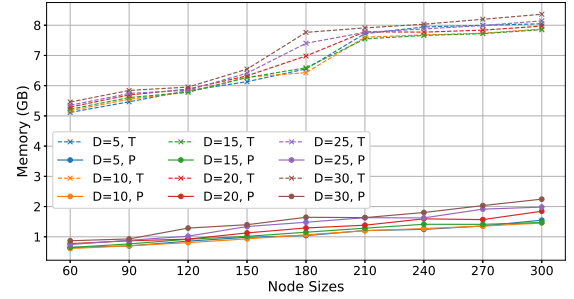
Fig. 8: Memory allocation on Random Regular Graph. P: curvature precomputation phase, T: GCNN training phase.
