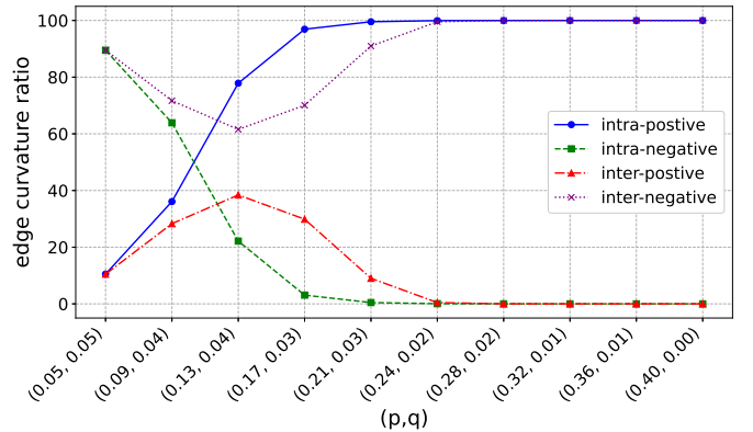
Fig. 10: Ollivier-Ricci curvature distribution in different clustering phases. intra-positive: proportion of intra-cluster edges with positive curvature, intra-negative: proportion of intra-cluster edges with negative curvature, inter-positive: proportion of inter-cluster edges with positive curvature, inter-negative: proportion of inter-cluster edges with negative curvature.
