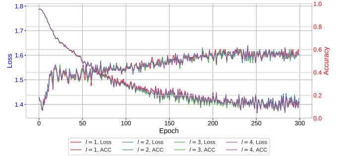
Fig. 11: Trends in validation loss and accuracy in different ricci flow iteration l on ENZYMES dataset.
