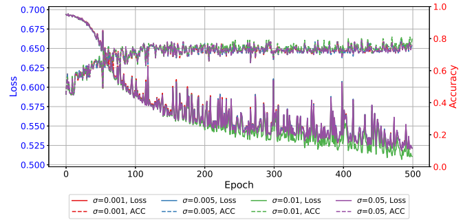
Fig. 14: Trends in validation loss and accuracy in different stop threshold \delta on ENZYMES dataset.
