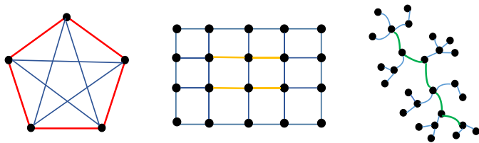
Fig. 1: Example of Ricci curvature on graphs. From left to right, the Ricci curvature of the red edges are positive, the orange edges are zero, and negative for the green edges in tree-structure graph, respectively. However, all edges have same weight 1.
