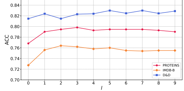
Fig. 3: The prediction accuracy of RicciPool under different Ollivier-Ricci flow iterations l with the same number of clusters K = 32 .
