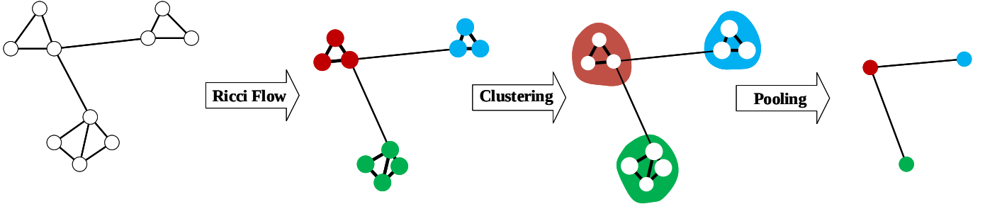
Fig. 2: Ollivier Ricci flow based graph pooling model.
