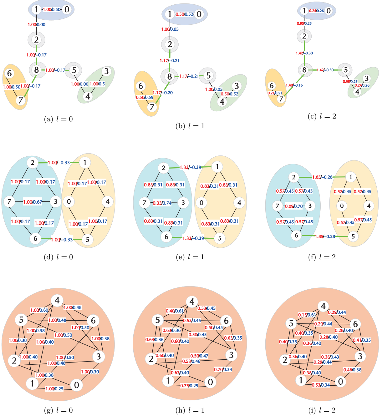
Fig. 6: Visualization of the Ollivier-Ricci flow in RicciPool, using three real example graphs from the ENZYMES (first row, ID 351, referred to as graph A below) and PROTEINS datasets (IDs 1084 and 412, referred to as graphs B and C below). Figures a-c, d-f, and g-i show the states of graphs A, B, and C after 0, 1, and 2 iterations of the Ollivier-Ricci curvature flow, with the numbers on the edges indicating the distances between nodes. The subgraphs with different background colors represent different communities. The lengths of the edges represent the edge weights. The black lines on the edges indicate positive curvature, while the green lines indicate negative curvature.
