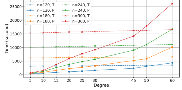
Fig. 7: Wall-clock time allocation on Random Regular Graph. P: curvature precomputation phase, T: GCNN training phase.
