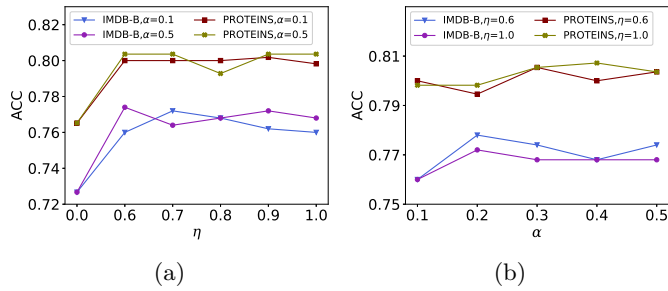
Fig. 5: Performance on different \eta (left) and \alpha (right) values for dataset IMDB-B and PROTEINS.
