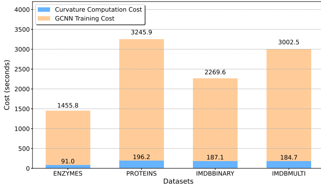
Fig. 9: Costs on curvature precomputation and GCNN training.
