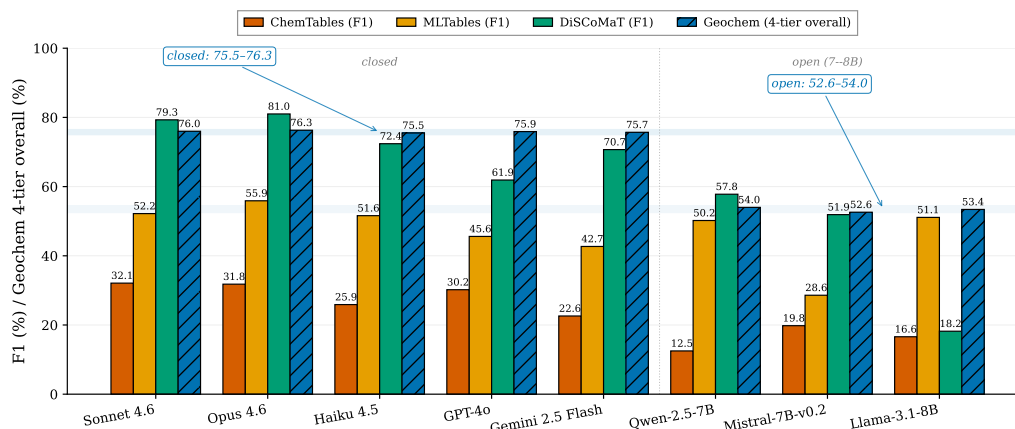
Figure 3: Per-backbone score across the four tasks (corresponding to Table 4): strict tuple- F_1 (%) for CHEMTABLES/MLTABLES/DiSCoMAT and four-tier Overall S (%) for GEOCHEM. The two metrics are distinct constructs and are not directly comparable across tasks.
