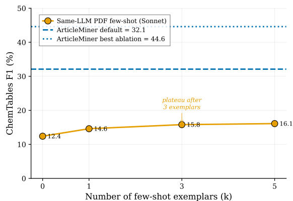
(b) CHEMTABLES few-shot F_1 vs. k -shot exemplars (Sonnet 4.6).
