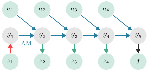
Figure 1: Action-conditioned hidden Markov model for a visual trace of length T = 5 representing the overall model to learn. Grey nodes indicate hidden symbolic state variables and green nodes indicate input actions and images. The perception model p_{\theta}(S_1 | z_1) predicts the belief of the initial state. The probabilistic action model AM and the observed grounded actions \mathbf{a} produce the successor states through p_{\theta_{AM}}(S_{t+1} | S_t, a_t) . The emission model p_{\theta}(z_t | S_t) measures the agreement between the states and their associated images, while the final-state supervision compares the sampled endpoint s_5 with the observed description f .
