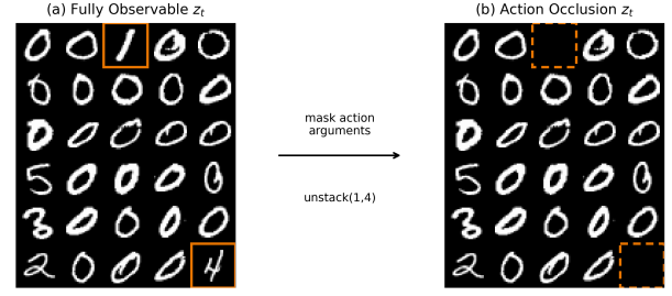
Figure 2: Action Occlusion in grid-based Blocks World. For unstack(1,4) , solid boxes mark the action arguments in the Fully observable case (O1) (left), while dashed boxes mark their masked locations under Action occlusion (O3) (right).
