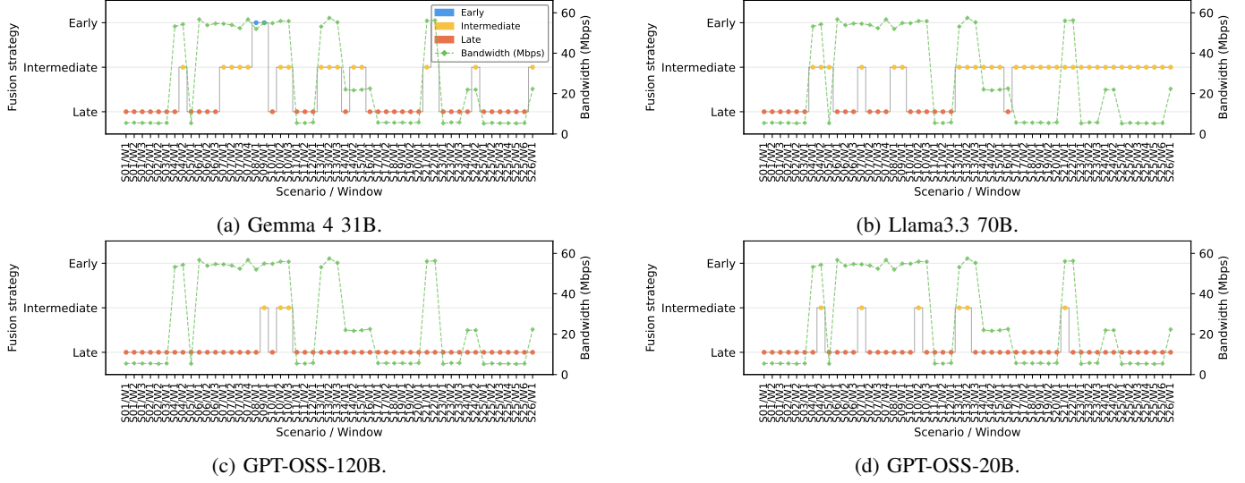
Fig. 6: CoAdapt-selected fusion strategy vs. available bandwidth.
