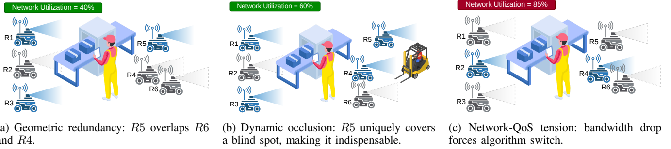
Fig. 1: Three snapshots of an IIoT robot swarm exposing distinct challenges in adaptive collaborative perception. Blue robots are active participants; gray robots are excluded.
