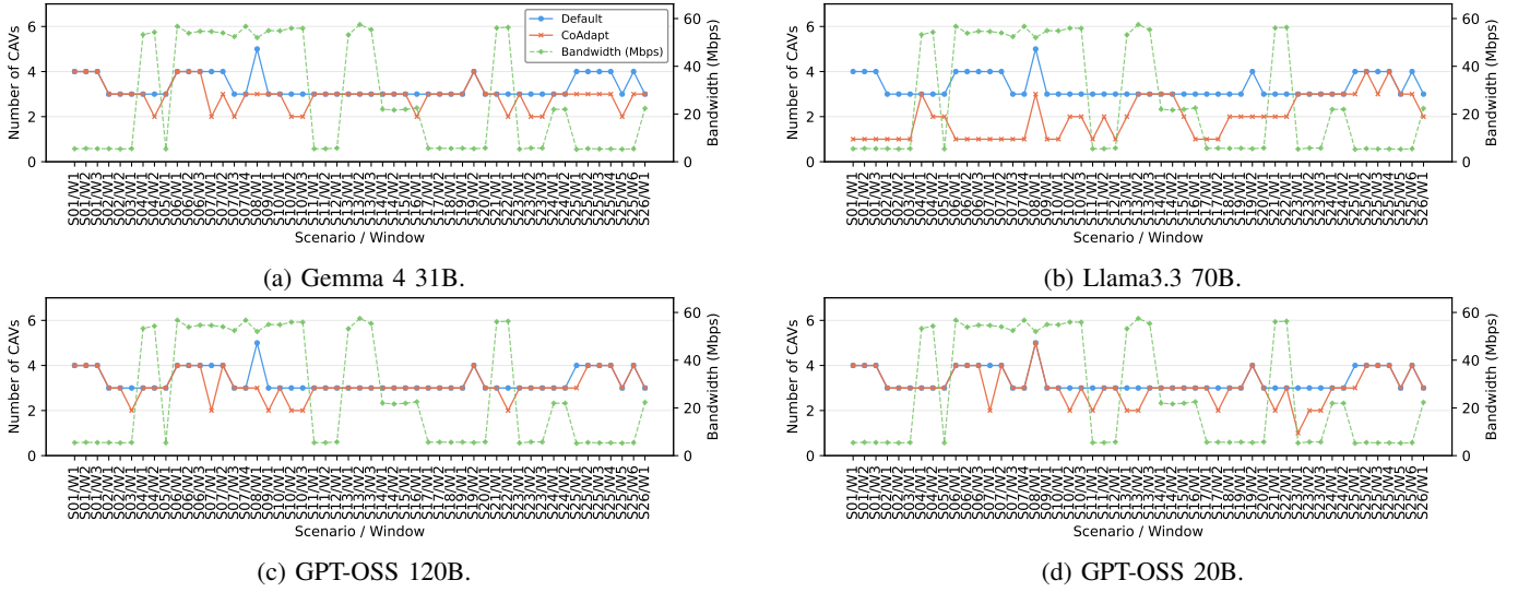
Fig. 4: Number of selected CAVs vs. network bandwidth.
