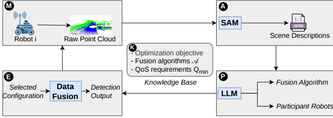
Fig. 3: CoAdapt's integration within the MAPE-K loop.
