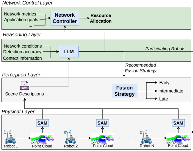
Fig. 2: The CoAdapt architecture.
