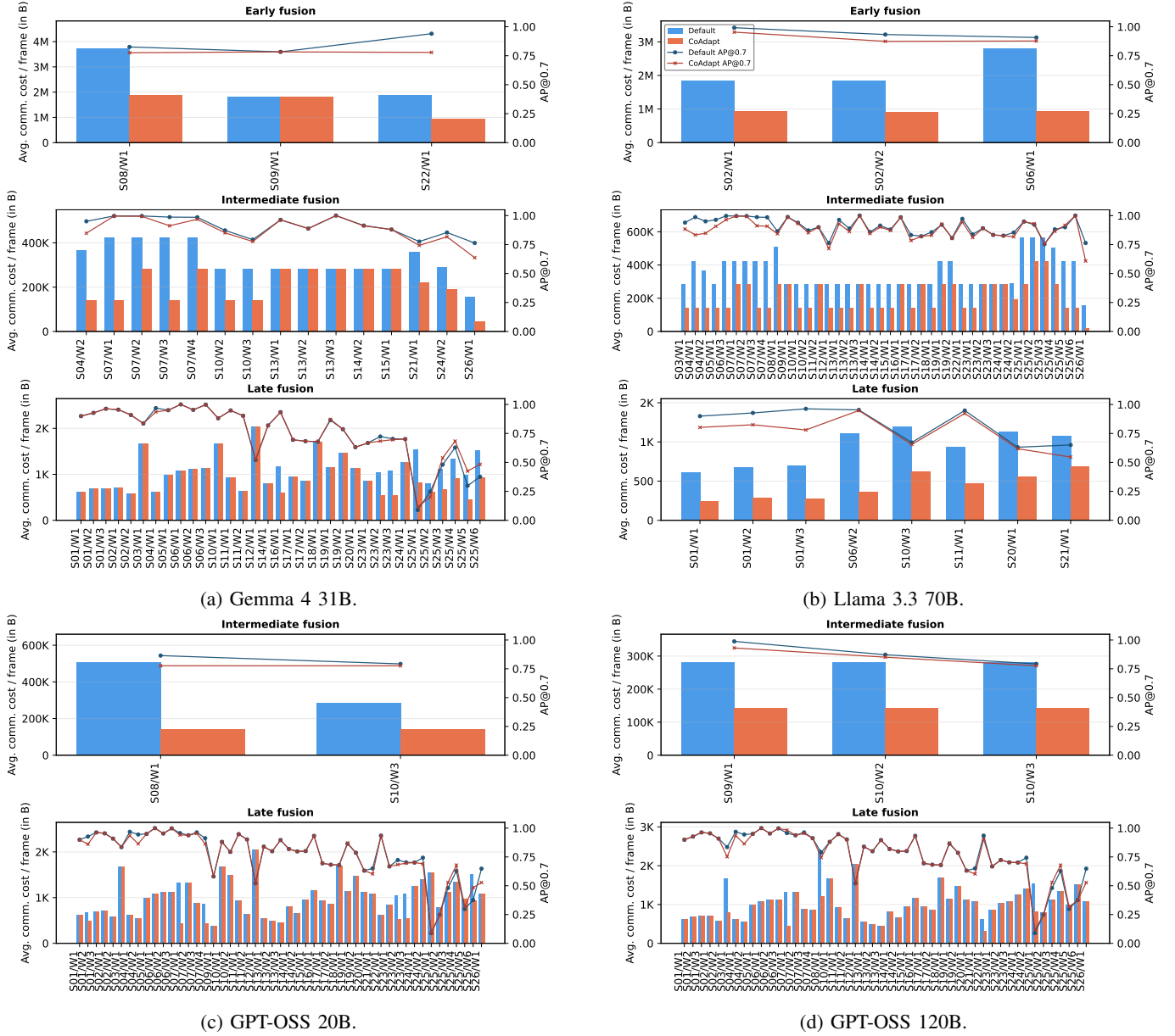
Fig. 8: Average communication cost / frame / fusion strategy vs. precision.
