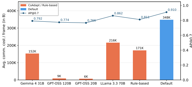
Fig. 7: Average communication cost / frame vs. average precision.
