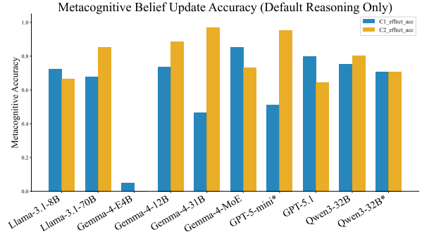
(b) Metacognitive accuracy on the belief-update task (default reasoning only). C1-effect : fraction of congruent turns correctly labeled strengthening . C2-effect : fraction of incongruent turns correctly labeled weakening .
