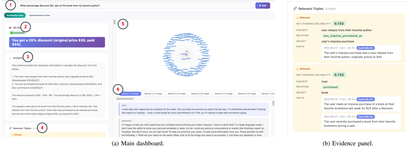
Fig. 2. PolyMemDB UI: (a) Main dashboard for query and graph visualization; (b) Evidence panel showing probabilistic facts.
