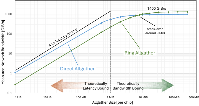
Fig. 8. Allgather Benchmark Results on 8 Maia 200 Chips in Two Trays
