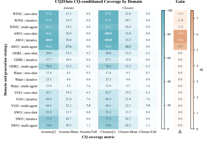
(b) CQ-conditioned coverage and gain.
