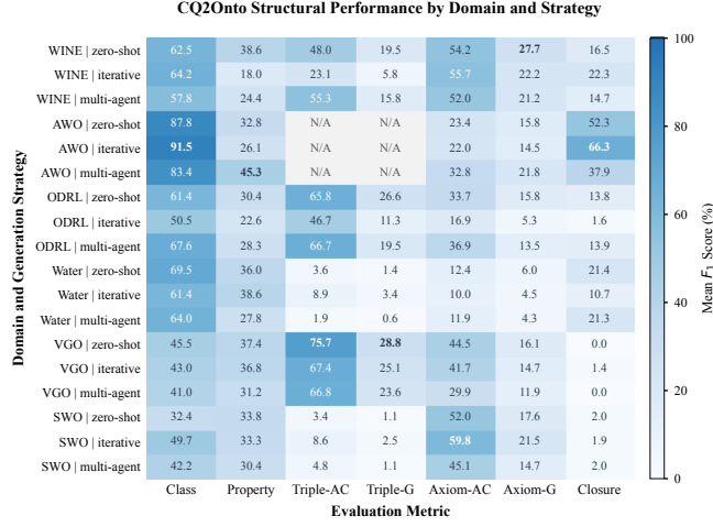
(a) Structural performance ( F_1 ).
