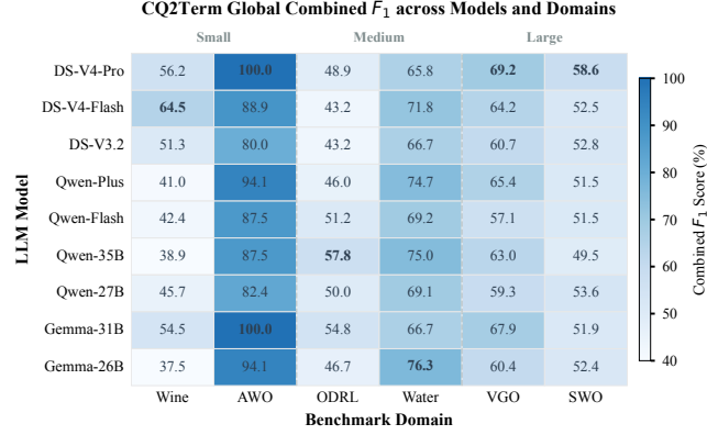
(a) Overall term F_1 by model and domain.
