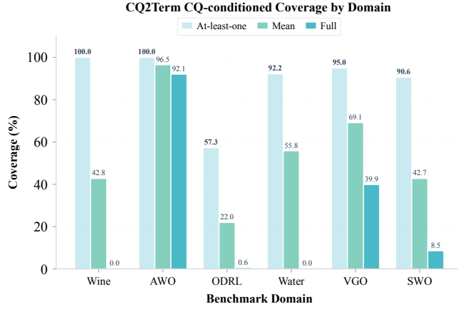
(b) CQ-conditioned coverage averaged over 9 LLMs.
