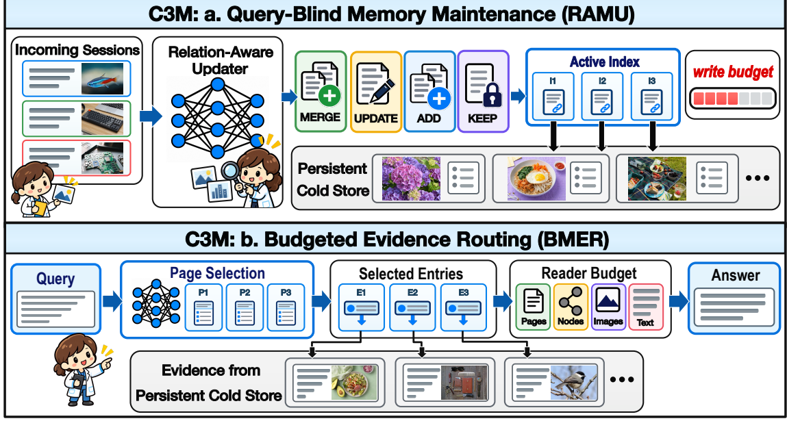
Fig. 2. Overview of C3M. (a) During query-blind memory maintenance, RAMU applies relation-aware MERGE, UPDATE, ADD, or KEEP actions to incoming multimodal sessions. Compact, provenance-linked entries are maintained in the active index under a fixed write budget, while original evidence is preserved in the persistent Cold Store. (b) Given a query, BMER selects index pages (P) and entries (E), then retrieves linked Raw Nodes and original images from the Cold Store under a joint reader budget over pages, nodes, images, and text for answer generation.
