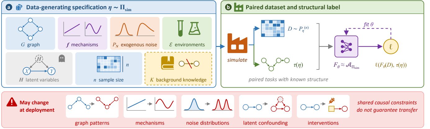
Fig. 6. Generation of training datasets and structural labels. (a) A data-generating specification \eta \sim \Pi_{\text{sim}} includes a graph, mechanisms, exogenous noise, environments, latent variables, sample size, and optional background knowledge. (b) The simulator generates a dataset D and structural label \tau(\eta) from this specification to train F_\theta . The bottom row illustrates factors that may change at deployment. Sharing causal constraints between training and test distributions alone does not guarantee transfer.
