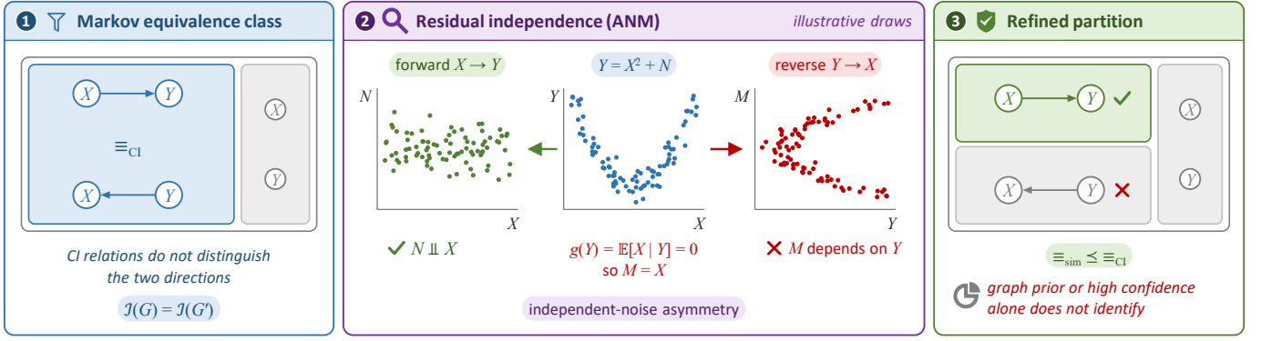
Fig. 7. Functional restrictions can distinguish Markov-equivalent directions. The illustrative draws use X \sim \mathcal{U}[-2, 2] and Y = X^2 + N , with independent N \sim \mathcal{N}(0, 0.4^2) . The forward residual is N . Symmetry gives the reverse population regression g(Y) = \mathbb{E}[X | Y] = 0 , whose residual M = X depends on Y . Identification requires the functional-model conditions; a graph prior or high confidence alone does not supply them.
