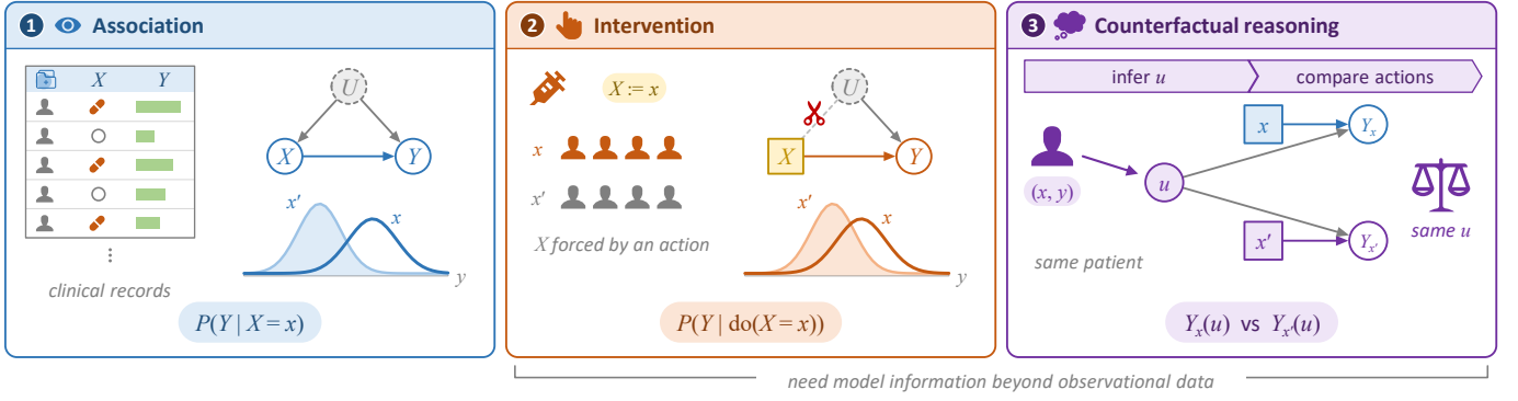
Fig. 2. Three causal queries, illustrated by treatment X and recovery Y . Clinical records describe association; intervening replaces the treatment mechanism by X = x . Counterfactual reasoning uses a causal model to infer an exogenous context u and compare actions for the same patient, Y_x(u) versus Y_{x'}(u) . The table and curves are schematic. Observational data alone need not identify the model information required by the latter two queries.
