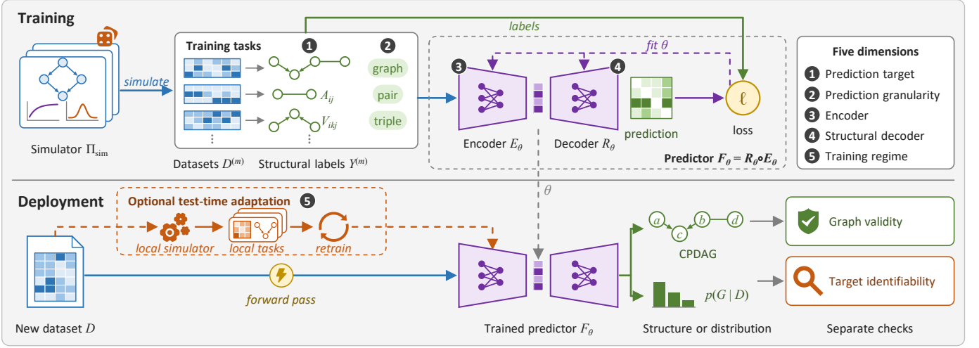
Fig. 1. A common SCD workflow. Training samples causal models, generates paired datasets and structural labels, and fits an encoder E_{\theta} and decoder R_{\theta} . The prediction target and granularity specify whether labels describe complete graphs or local units, such as pairs and triples. Deployment encodes a new dataset and decodes a structure or a distribution over structures; the illustrated output is a CPDAG. Optional test-time adaptation fits a local simulator to the new dataset, generates local tasks, and retrains the predictor. Graph validity and target identifiability require separate checks. Numbered badges mark the five dimensions used to compare methods.
