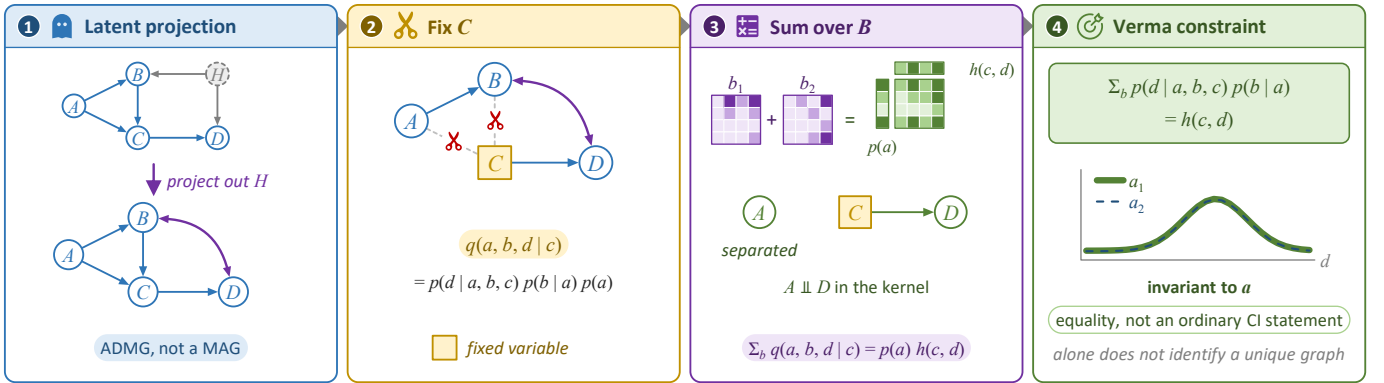
Fig. 8. The Verma constraint in four steps. Projecting out a common cause of B and D gives the bidirected edge in the ADMG. Fixing C removes its incoming edges and yields a derived kernel. Summing this kernel over B separates A and D conditional on fixed C ; equivalently, the displayed weighted sum is invariant to a . The squares denote fixed variables; heat maps are schematic. This constraint alone does not establish a uniquely identified graph.
