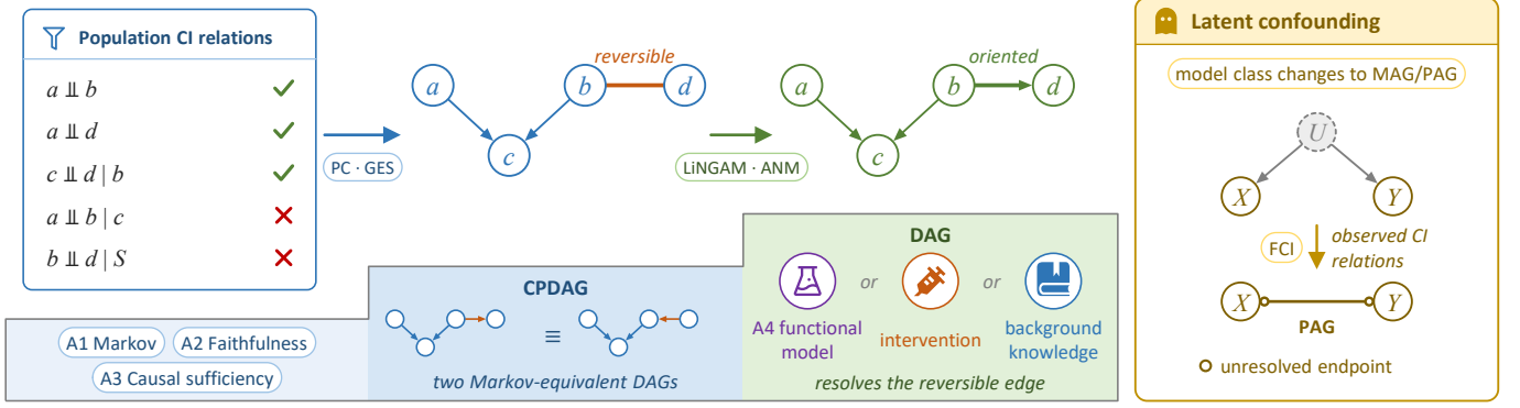
Fig. 4. Graph targets under different assumptions. In an observed DAG satisfying A1–A3, population CI relations identify a CPDAG. The example a \rightarrow c \leftarrow b with b \rightarrow d has one reversible edge. Additional direction information can resolve it. Allowing latent confounding changes the model class to MAG/PAG semantics; circles in the two-variable PAG indicate unresolved endpoints. Chips on the arrows name representative algorithms.
