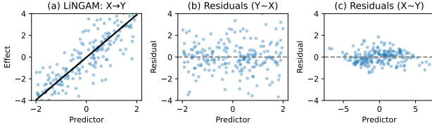
Fig. 3. LiNGAM asymmetry illustrated by 200 samples with X \sim \mathcal{U}[-2, 2] , Y = 2X + \varepsilon , and independent \varepsilon \sim \text{Lap}(0, 1) . The population forward noise is independent of X , whereas the population reverse linear-regression residual depends on Y . The plots show fitted finite-sample residuals and illustrate this asymmetry; they are not independence tests.
