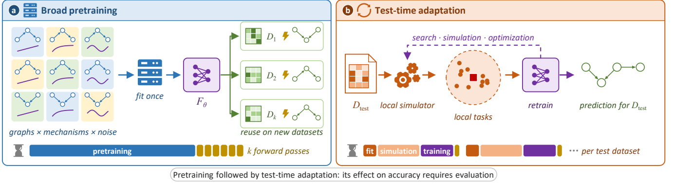
Fig. 5. Training and deployment costs for broad pretraining and test-time adaptation. (a) One predictor is trained on diverse simulated tasks and reused across datasets. (b) A local simulator is fitted to a test dataset, then generates local tasks for retraining the predictor. Test-time adaptation adds simulation and training costs for each test dataset. Broad pretraining can also be followed by test-time adaptation; its effect on prediction accuracy requires evaluation. Cost bars are schematic.
