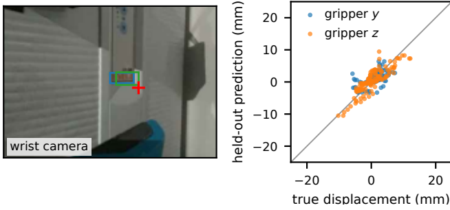
Fig. 9. Example of Codex’s analysis: learning jaw alignment to the handle. A regression model maps wrist-camera label-feature residuals to end-effector displacement toward the demonstrated closing pose. Left: detections before (blue) and after (green) lateral correction, with the goal in red. Right: held-out predicted versus true lateral displacement in the gripper frame. Redrawn from saved trial data and an offline regression evaluation.
