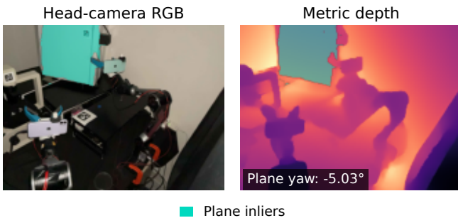
Fig. 10. Example of Codex’s analysis: door orientation from OpenCV tag-based pose estimation and a NumPy RANSAC plane fit. Overlays show plane inliers; yaw is estimated in the robot frame. Rendered by rerunning the evolved program on saved trial RGB-D data.
