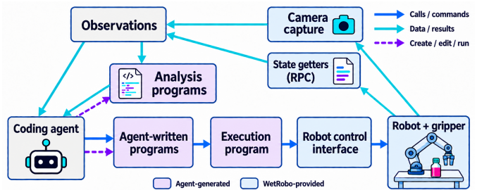
Fig. 3. How the coding agent observes and controls the robot during task performance.
