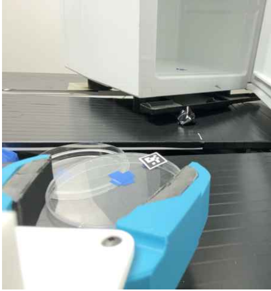
Fig. 4. Wrist-camera view of the lifted Petri lid held between the jaws.
