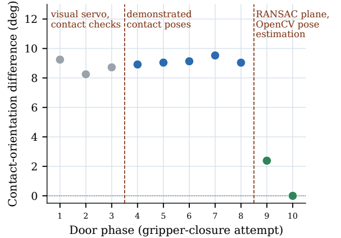
Fig. 8. Pre-close gripper orientation across recorded Lab X door attempts, relative to the successful final attempt.
