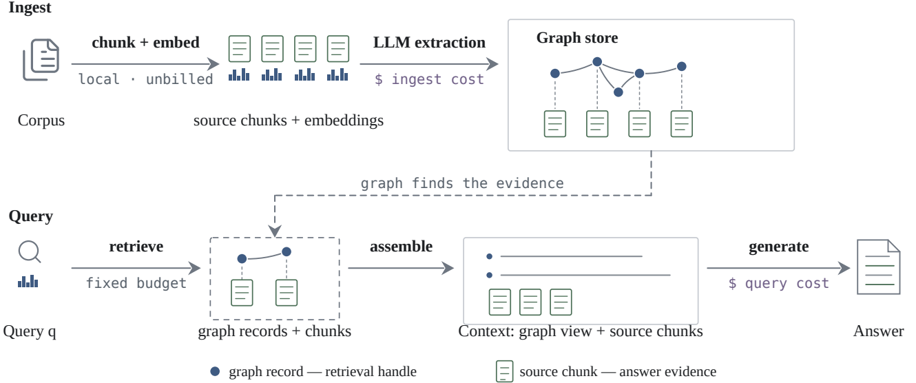
Figure 1: EffiRAG pipeline. Extracted entities and relations locate evidence; their supporting source chunks provide the original answer text.
