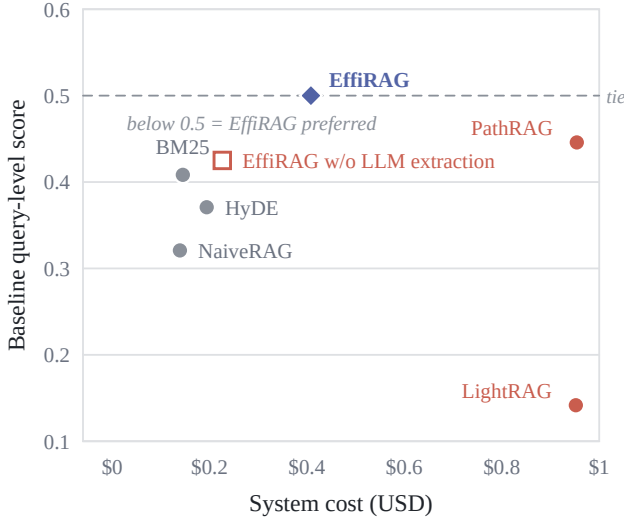
Figure 2: Cost and judged quality on UltraDomain.
