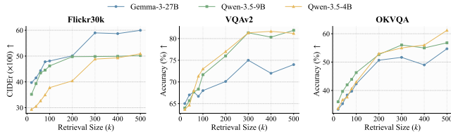
Figure 5: Effect of retrieval set size on COMIL. Performance generally improves as the retrieval set grows across Flick30k, VQAv2, and OKVQA, with diminishing gains at larger scales.
