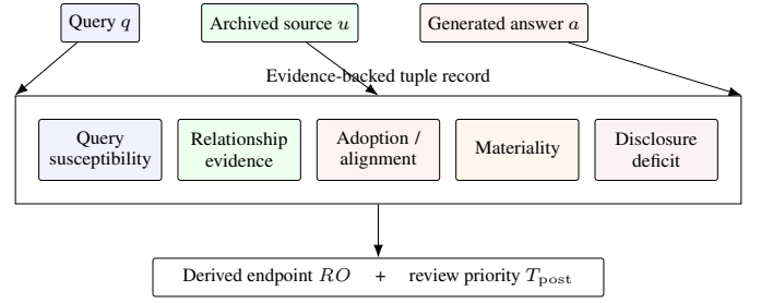
Fig. 1. Evidence flow for one tuple. The relationship, adoption, materiality, and disclosure fields resolve R_O ; d_Q affects review priority only. The reference checker consumes explicit judgments, not raw-text predictions.
