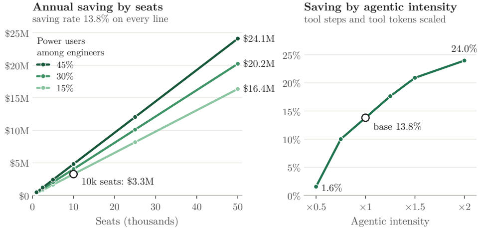
Figure 6: How the saving scales. Left: annual saving against seats for three shares of power users among engineers, at the same saving rate on every line. Right: saving against agentic intensity, tool steps and tool-result tokens scaled together.
