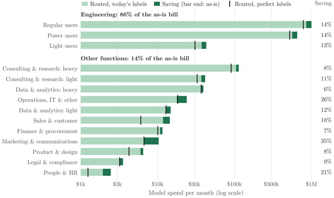
Figure 5: Monthly model spend by population segment. Each bar ends at the as-is bill; the green tail is the saving with today’s labels, the tick the routed bill with perfect labels. Engineering carries 86% of the bill; non-engineering segments save 6 to 35% of small bills.
