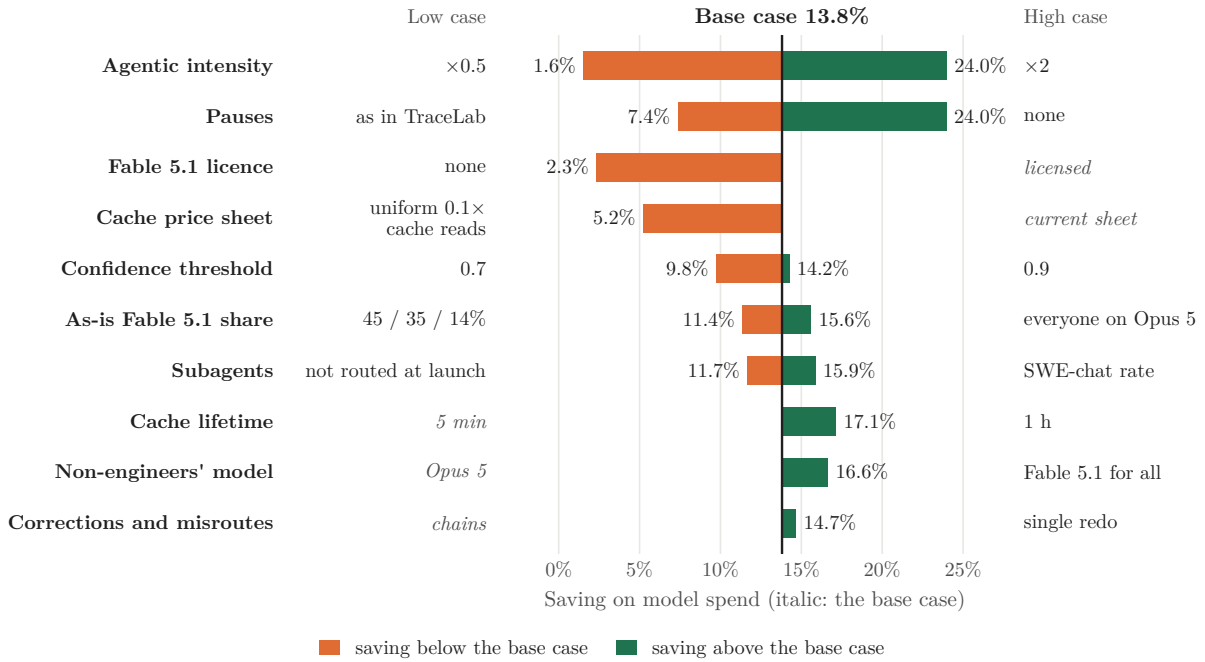
Figure 9: One-at-a-time sensitivities of the population saving, one row per driver with its low and high case; italic case names mark the base (base 13.8%; same labels and random draws). Orange bars run below the base, green bars above it. Table 4 lists every case.
