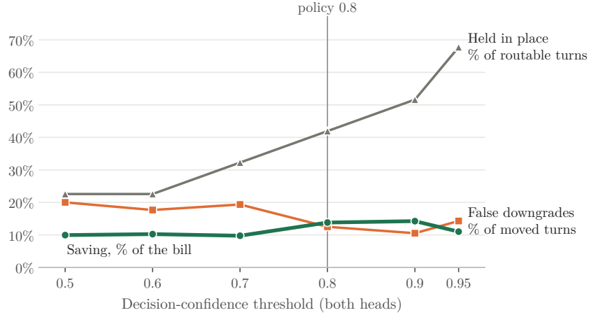
Figure 12: Saving, false-downgrade rate and hold rate against the decision-confidence threshold, applied to both of the classifier’s decision questions: the tier a turn needs and its dependence on the history.
