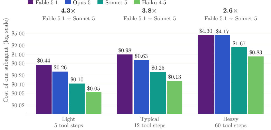
Figure 11: Cost of one subagent by model and activity profile (15k-token system prompt, 1.2k-token brief; tool results and output as in Appendix B). Subagents write their whole context once and read it a dozen times; the gap between the top model and the mid tier is largest for short subagents and narrows for very long ones.
