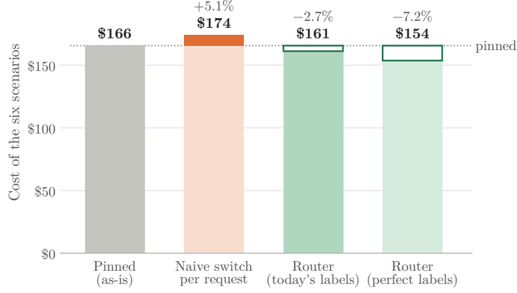
Figure 1: Six technical scenarios priced four ways: pinned, with naive per-request switching, and with the router on the live classifier’s labels and on perfect labels. The naive per-request switch pays a cold cache write on every move and, when the tags say the cheaper model was too weak, redoes the turn; the router runs small tasks in a separate lane and never rewrites the main conversation.
